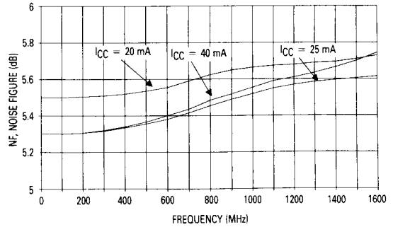
Figure 2. Noise Figure versus Frequency
