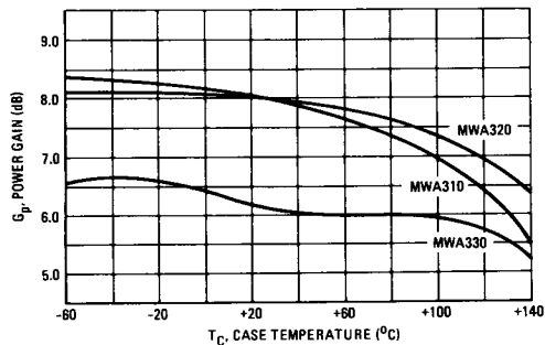
FIGURE 6 – POWER GAIN versus CASE TEMPERATURE f = 1000 MHz
