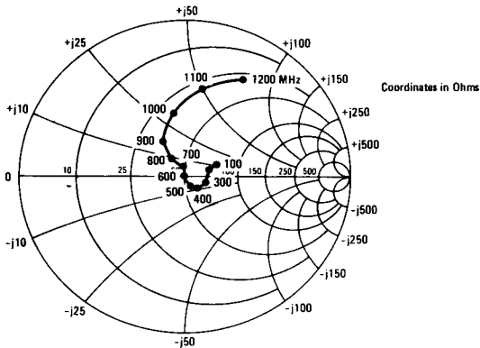
FIGURE 15 – OUTPUT IMPEDANCE versus FREQUENCY MWA330
