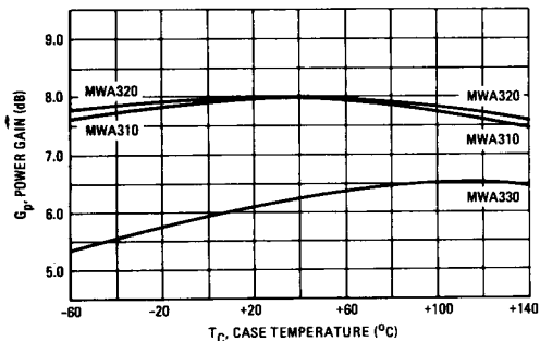
FIGURE 5 – POWER GAIN versus CASE TEMPERATURE f = 100 MHz
