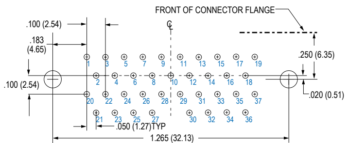
37 PIN MWDM-37PCBR
