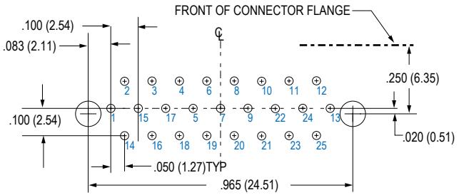
25 PIN MWDM-25PCBR
