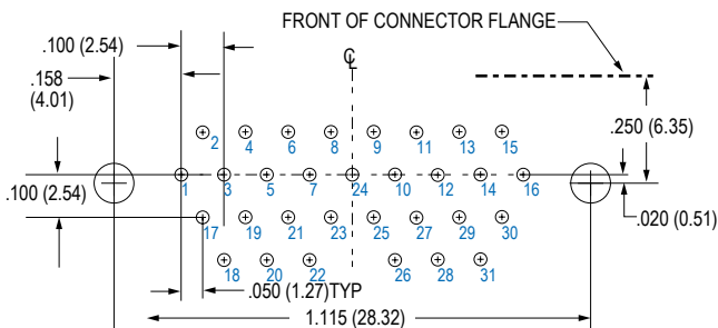
31 PIN MWDM-31PCBR
