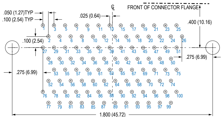
100 PIN MWDM-100PCBR
