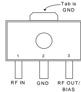
PK PACKAGE (Top View)
