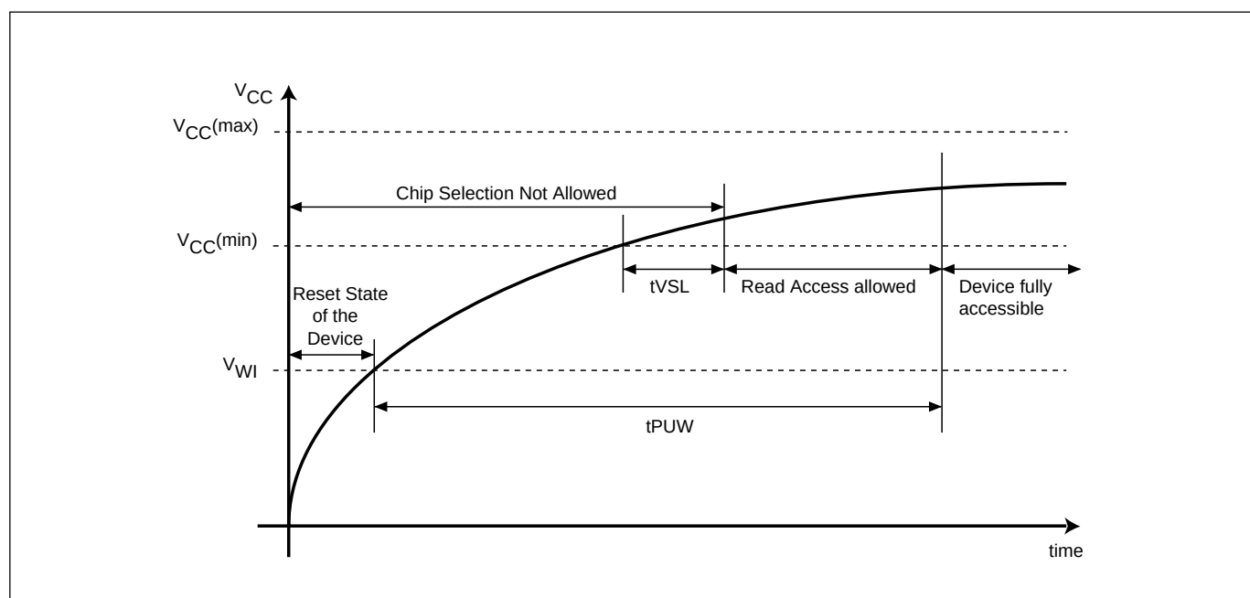
Figure 6. Power-up Timing
