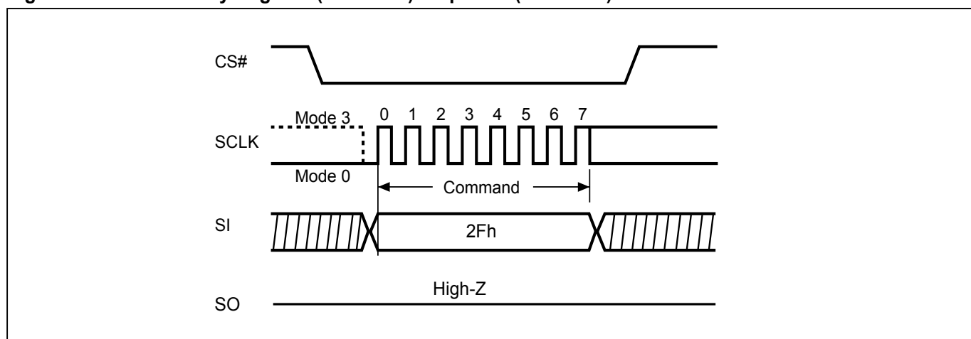
Figure 54. Write Security Register (WRSCUR) Sequence (SPI Mode)
