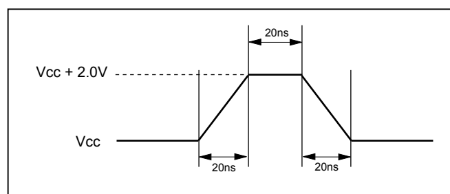
Figure 75. Maximum Positive Overshoot Waveform
