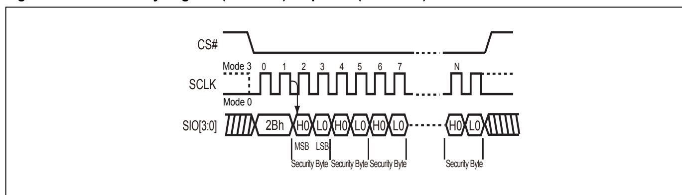
Figure 53. Read Security Register (RDSCUR) Sequence (QPI Mode)
