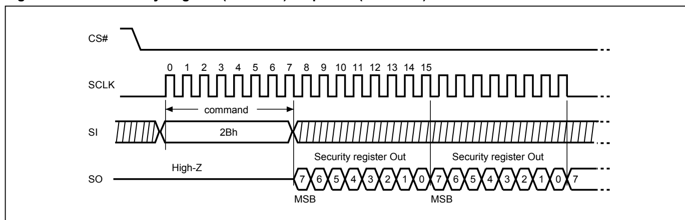
Figure 52. Read Security Register (RDSCUR) Sequence (SPI Mode)
