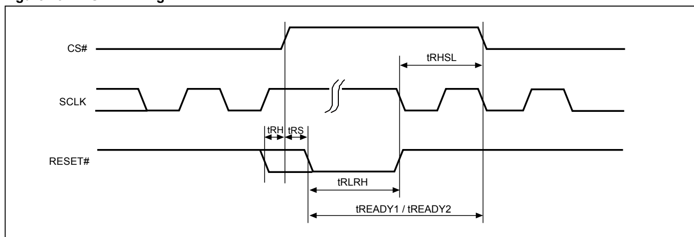
Figure 73. RESET Timing
