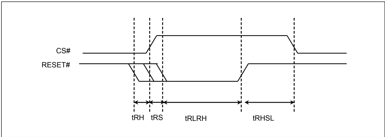
Figure 51. RESET Timing
