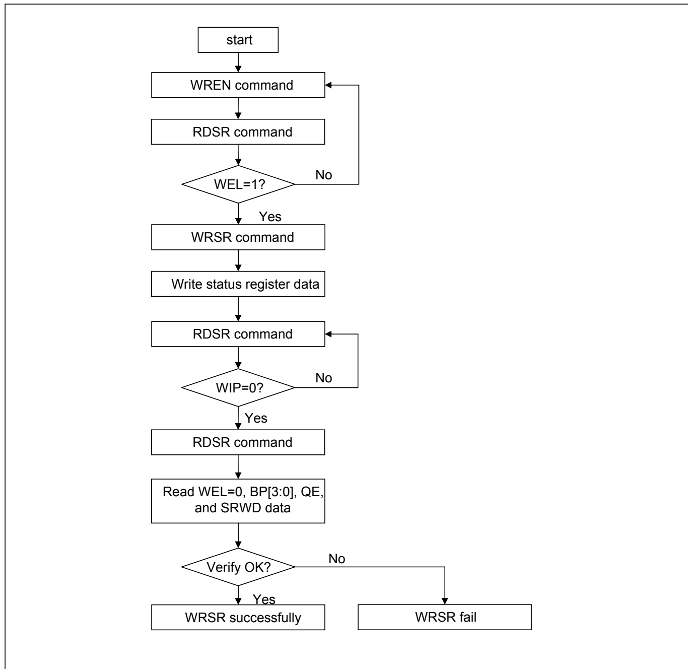
Figure 24. WRSR flow
