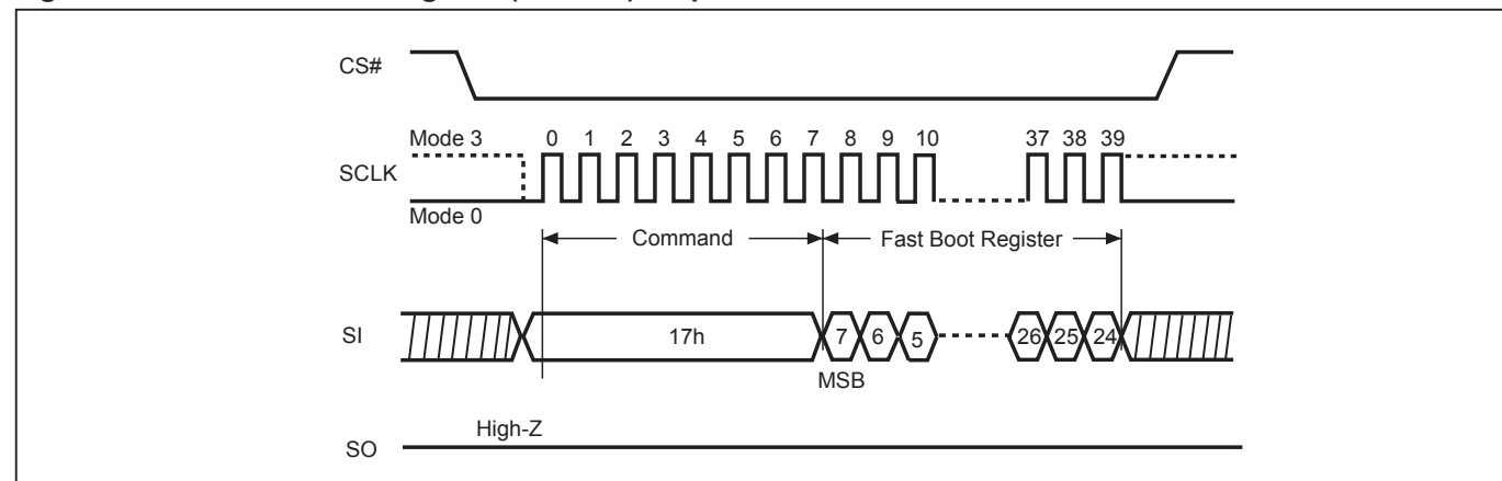
Figure 39. Write Fast Boot Register (WRFBR) Sequence
