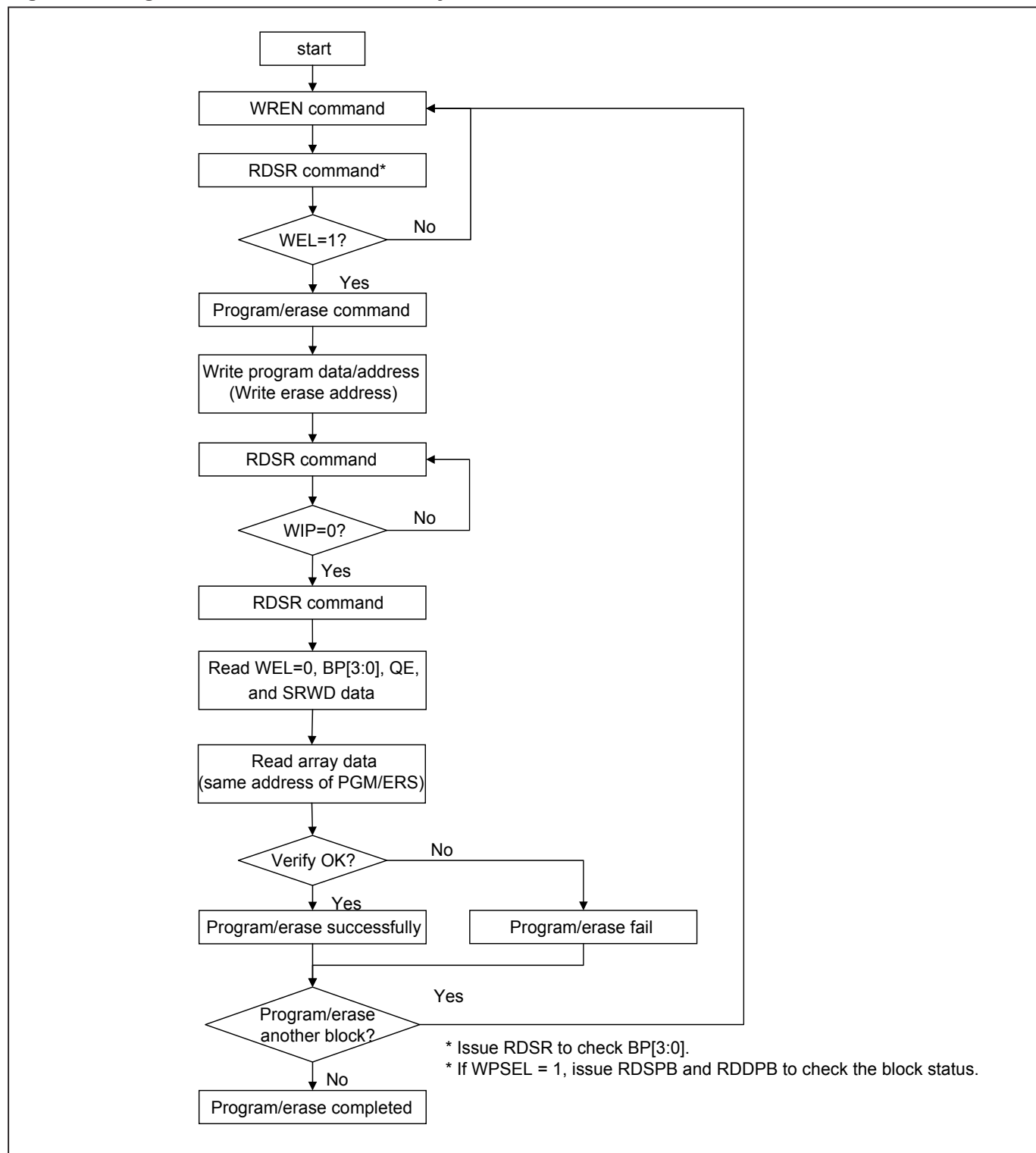
Figure 19. Program/Erase flow with read array data
