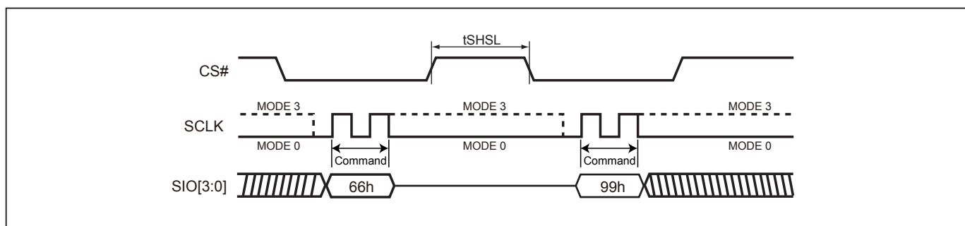
Figure 73. Reset Sequence (QPI mode)
