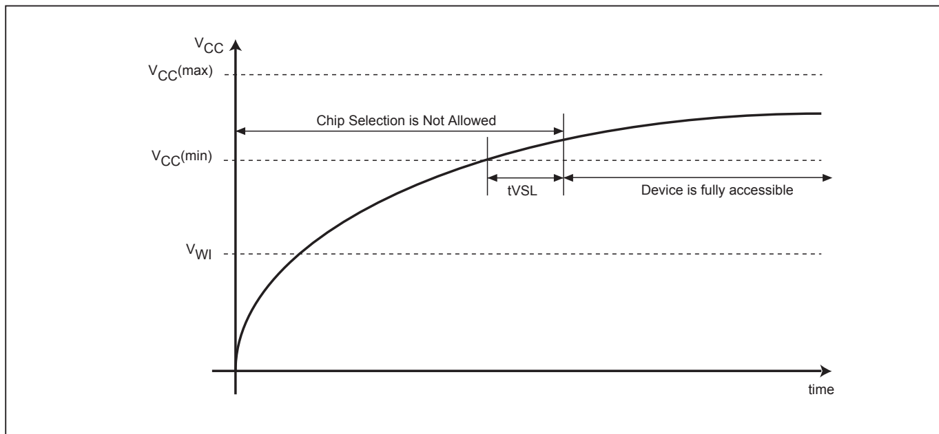
Figure 82. Power-up Timing
