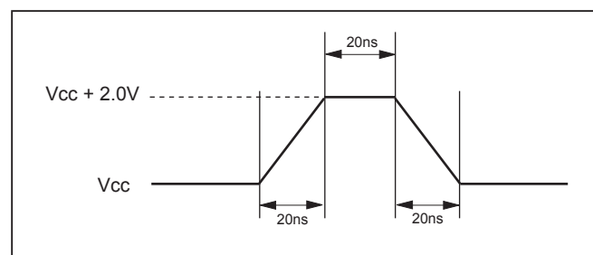
Figure 77. Maximum Positive Overshoot Waveform
