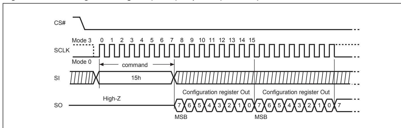
Figure 17. Read Configuration Register (RDCR) Sequence (SPI Mode)
