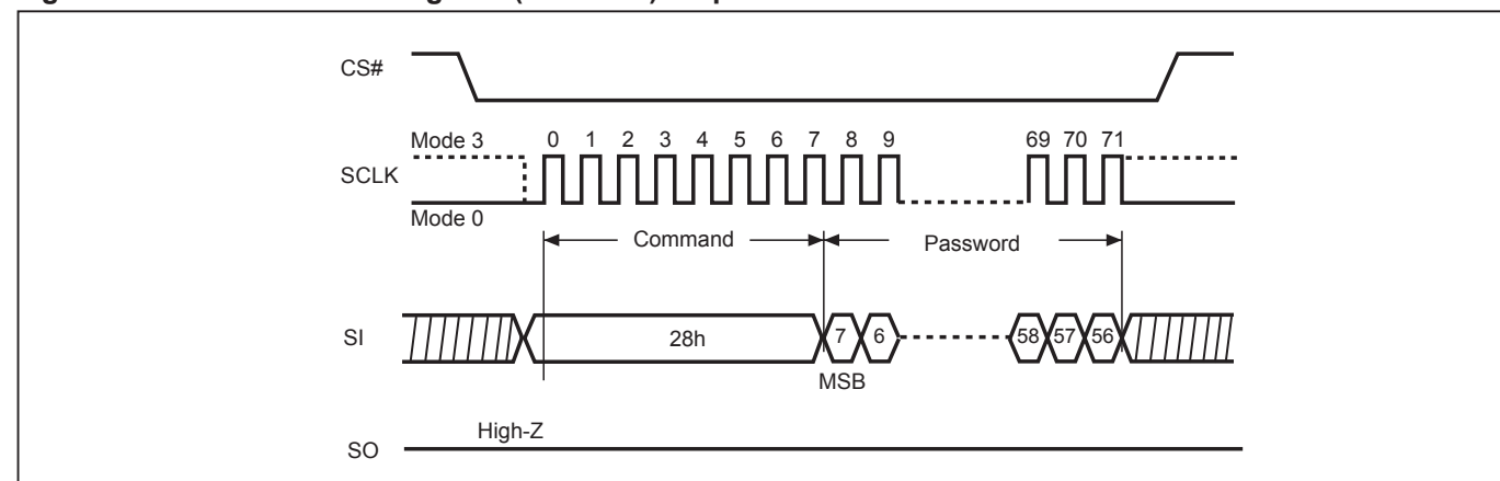
Figure 66. Write Password Register (WRPASS) Sequence
