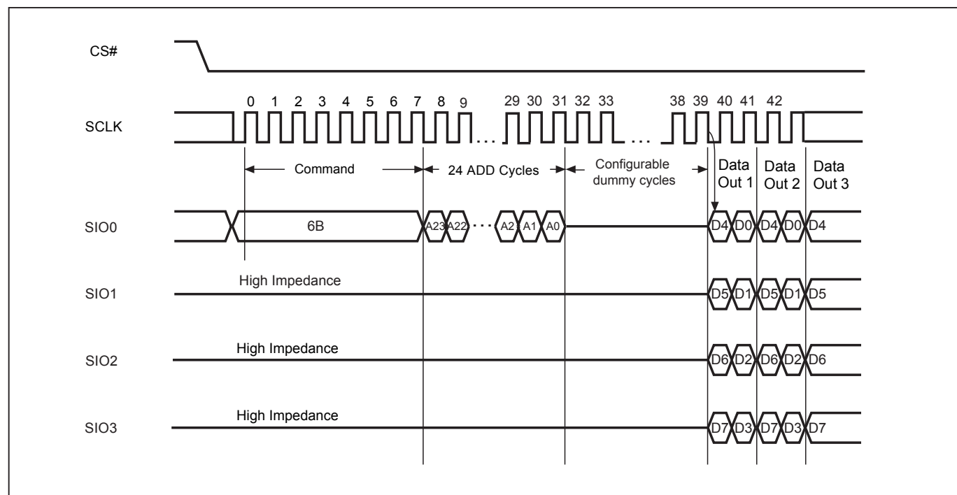
Figure 27. Quad Read Mode Sequence
