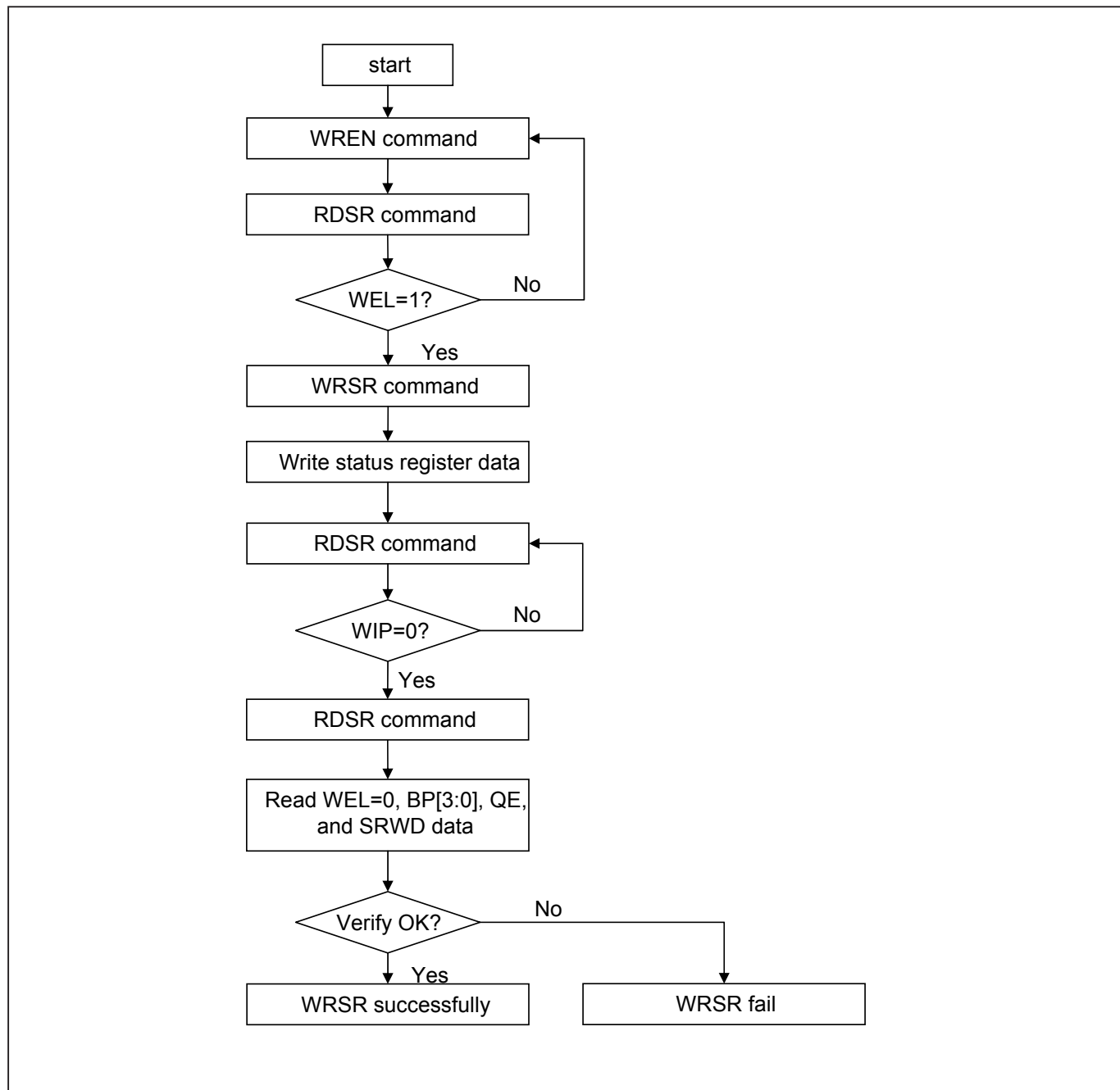
Figure 23. WRSR flow
