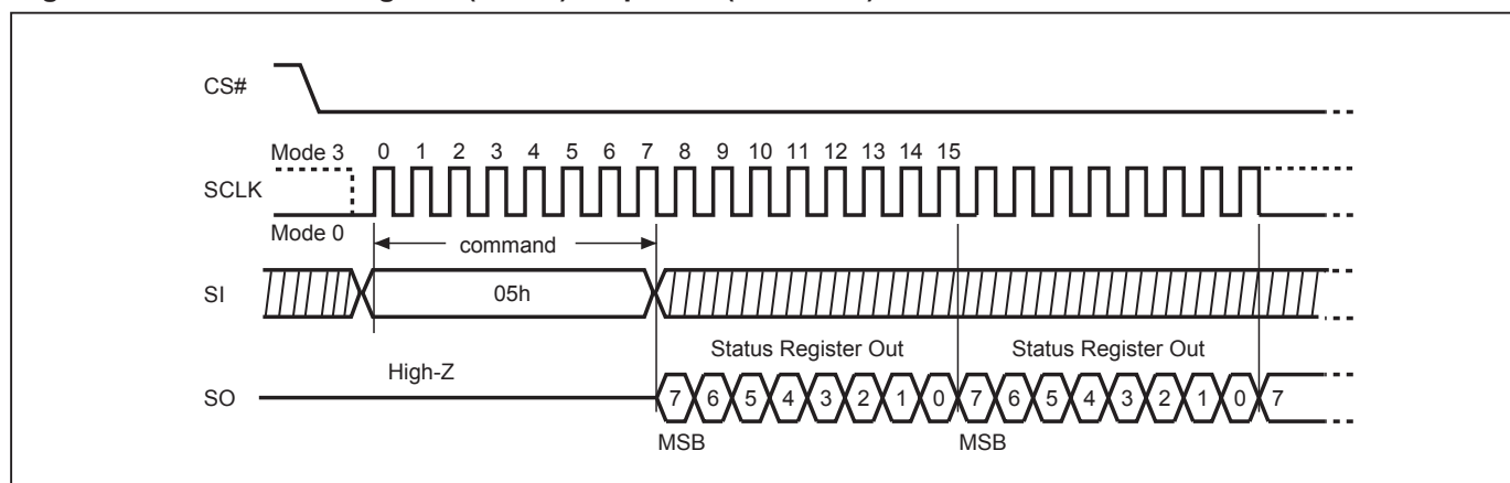
Figure 15. Read Status Register (RDSR) Sequence (SPI Mode)
