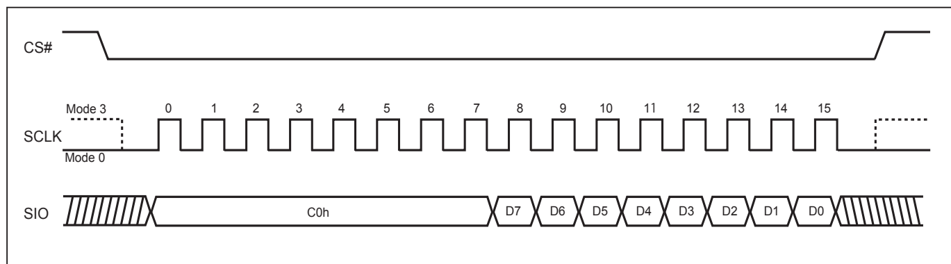
Figure 30. SPI Mode
