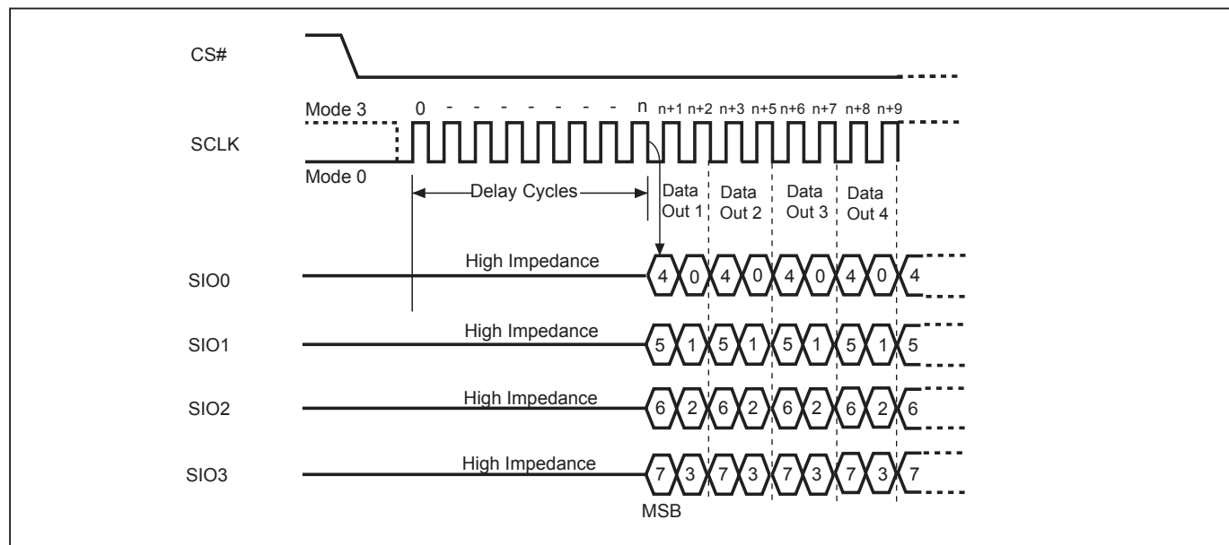
Figure 37. Fast Boot Sequence (QE bit =1)
