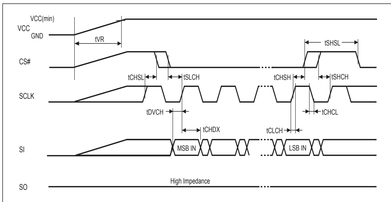
Figure 80. AC Timing at Device Power-Up
