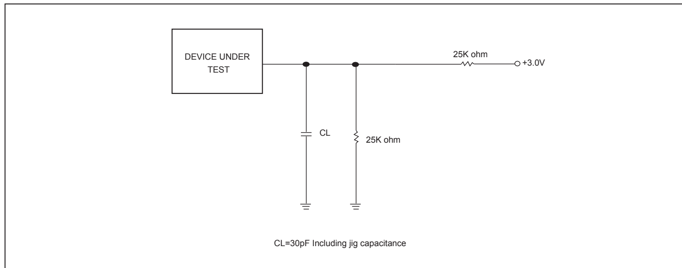
Figure 79. OUTPUT LOADING
