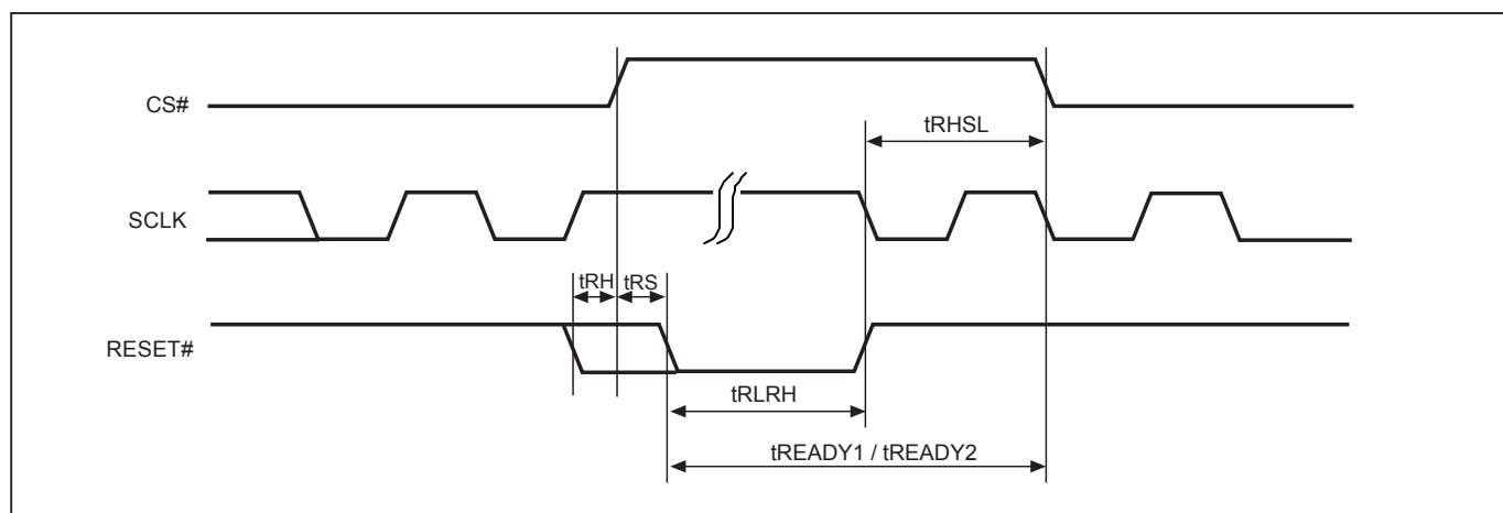
Figure 75. RESET Timing
