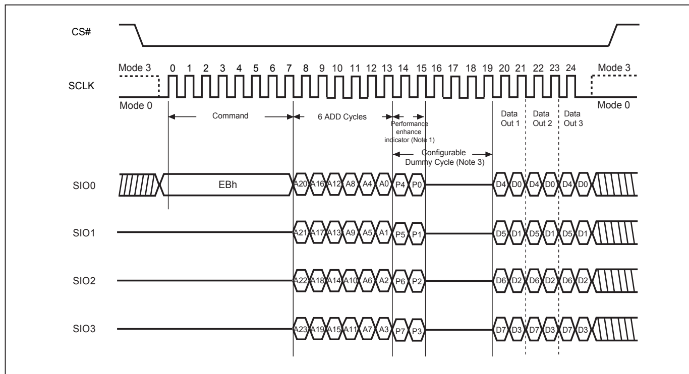
Figure 28. 4 x I/O Read Mode Sequence (SPI Mode)
