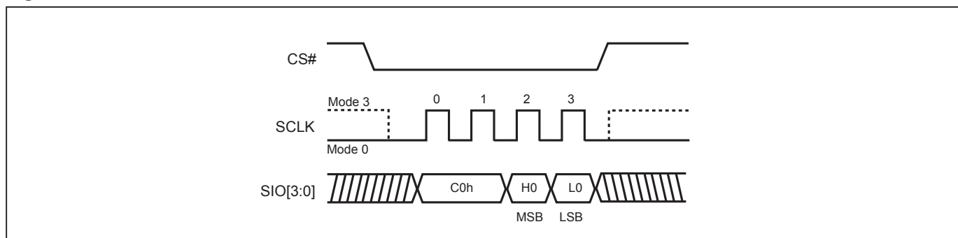
Figure 31. QPI Mode
