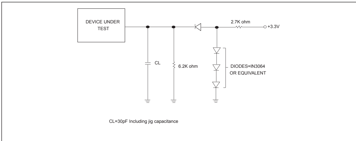
Figure 5. OUTPUT LOADING
