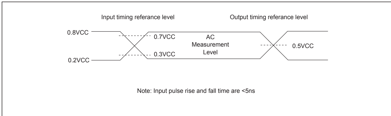
Figure 4. INPUT TEST WAVEFORMS AND MEASUREMENT LEVEL
