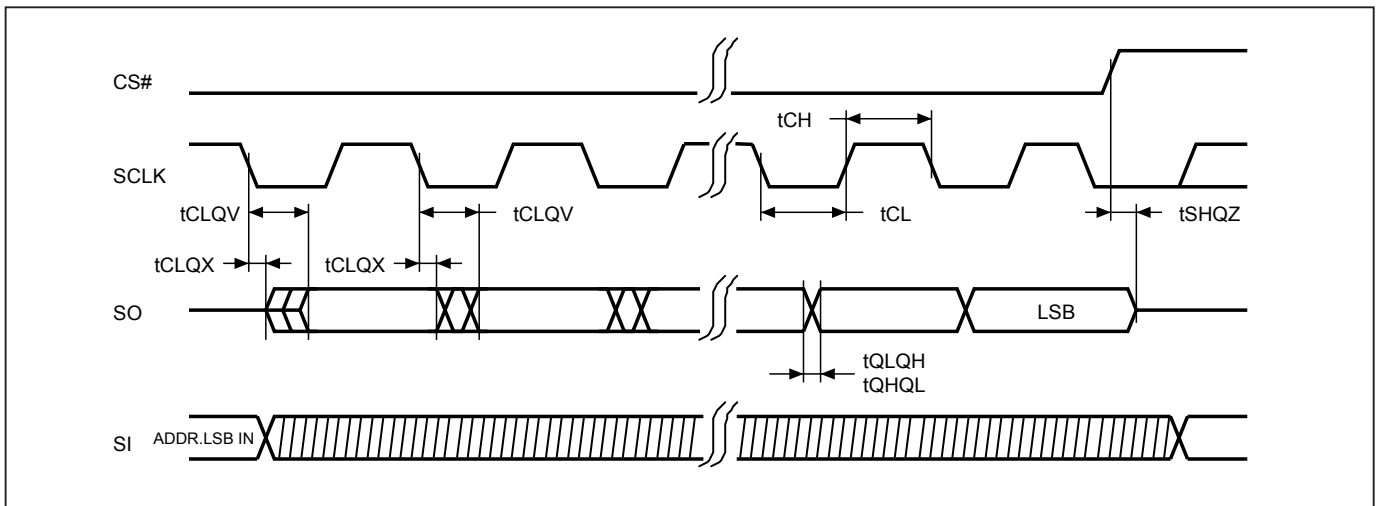
Figure 7. Output Timing
