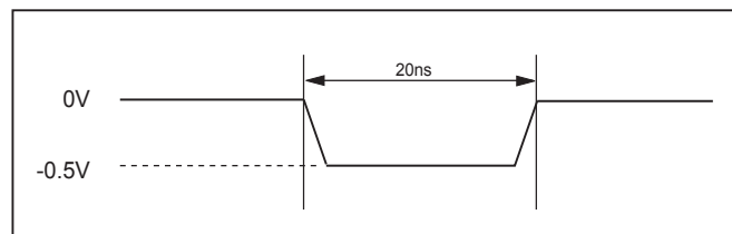
Figure 3. Maximum Negative Overshoot Waveform
