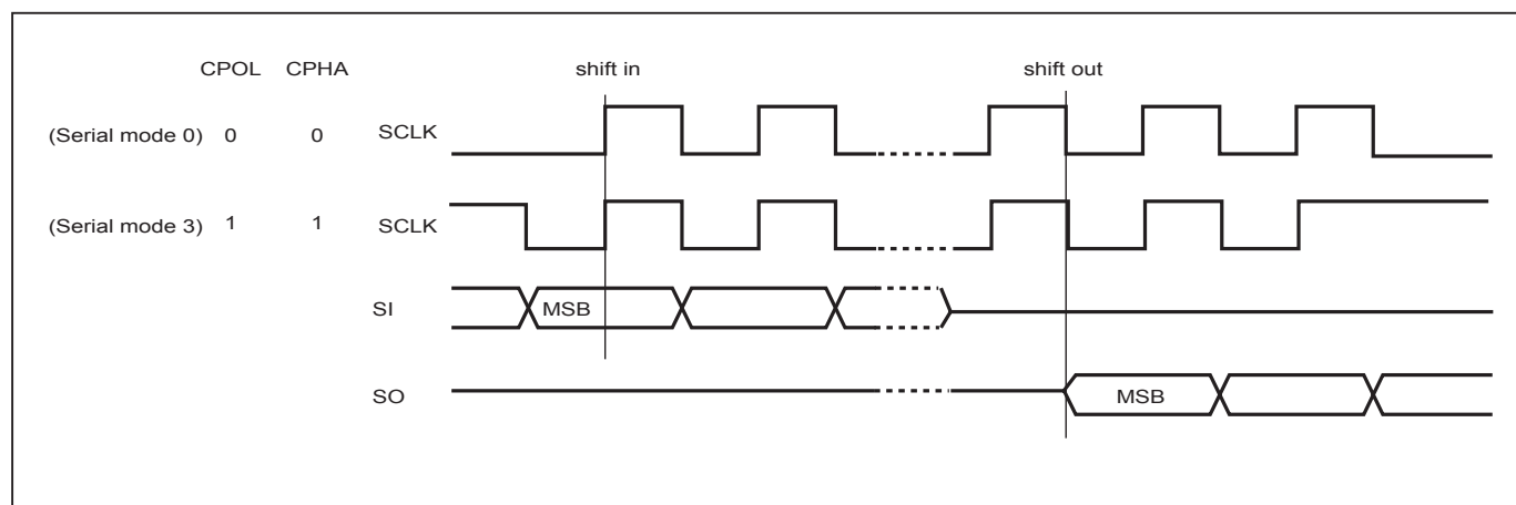
Figure 2. Serial Modes Supported
