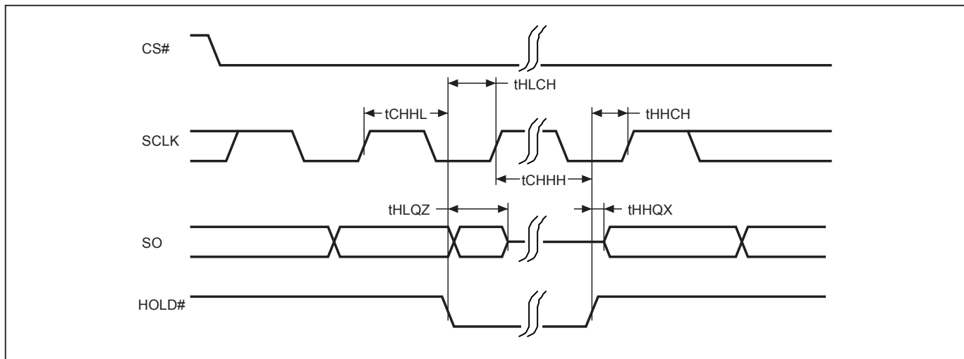
Figure 9. Hold Timing
