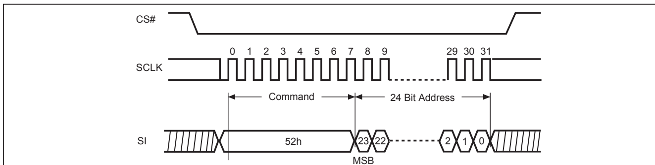
Figure 30. Block Erase 32KB (BE32K) Sequence (Command 52) (SPI Mode)
