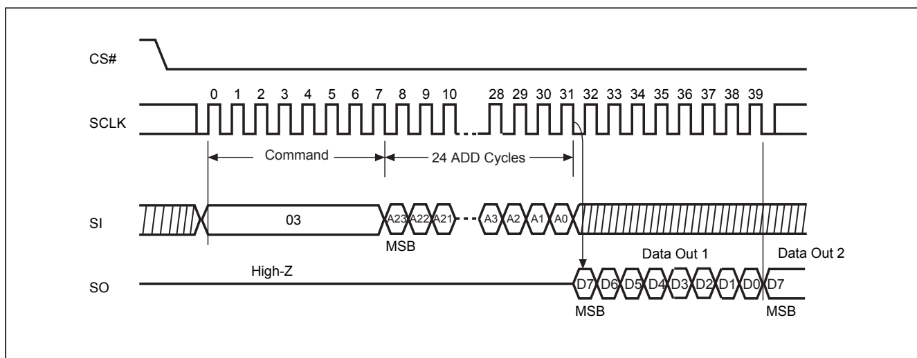
Figure 16. Read Data Bytes (READ) Sequence (Command 03)
