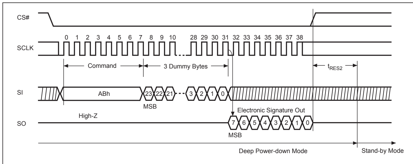
Figure 41. Release from Deep Power-down and Read Electronic Signature (RES) Sequence (Command AB)
