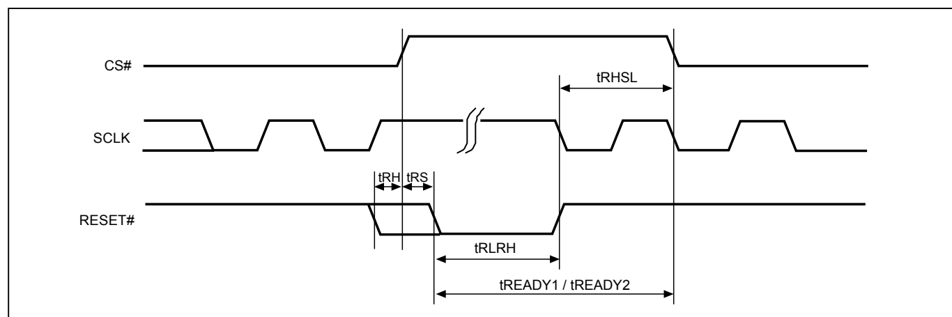
Figure 123. RESET Timing
