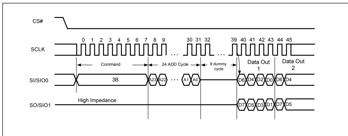
Figure 19. Dual Read Mode Sequence (Command 3Bh)
