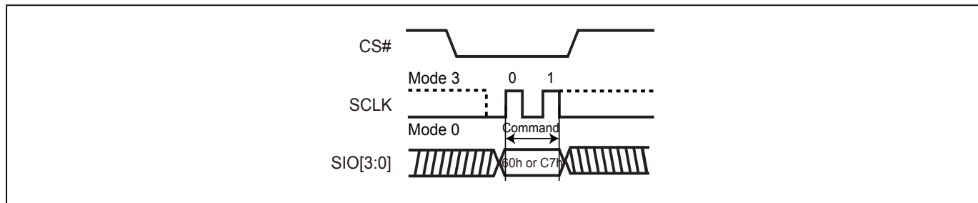
Figure 61. Chip Erase (CE) Sequence (QPI Mode)
