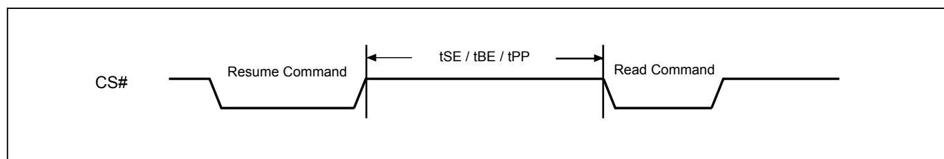
Figure 81. Resume to Read Latency
