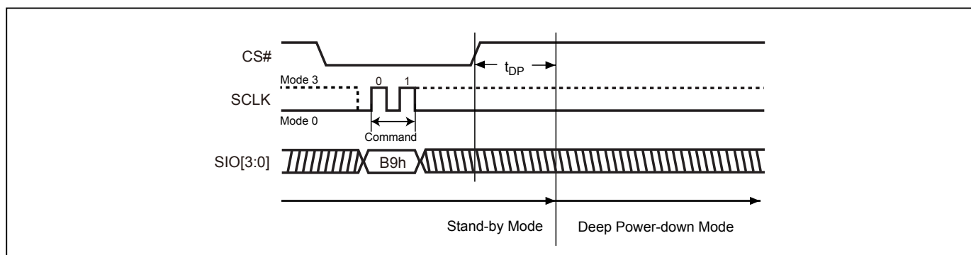
Figure 66. Deep Power-down (DP) Sequence (QPI Mode)
