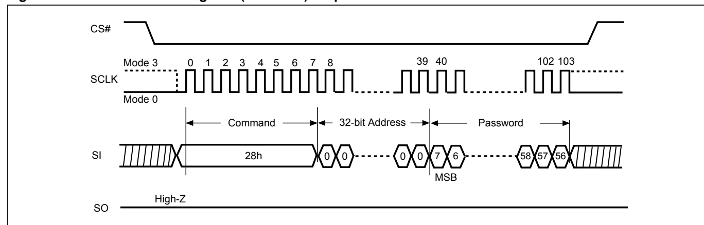
Figure 77. Write Password Register (WRPASS) Sequence
