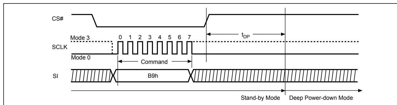
Figure 65. Deep Power-down (DP) Sequence (SPI Mode)
