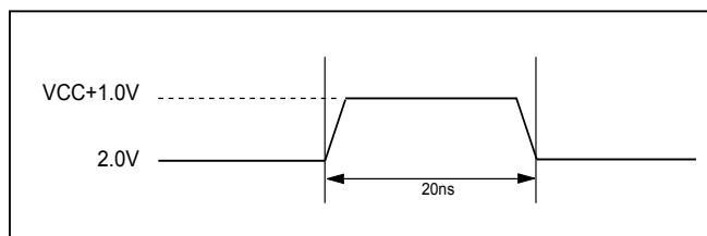
Figure 89. Maximum Positive Overshoot Waveform
