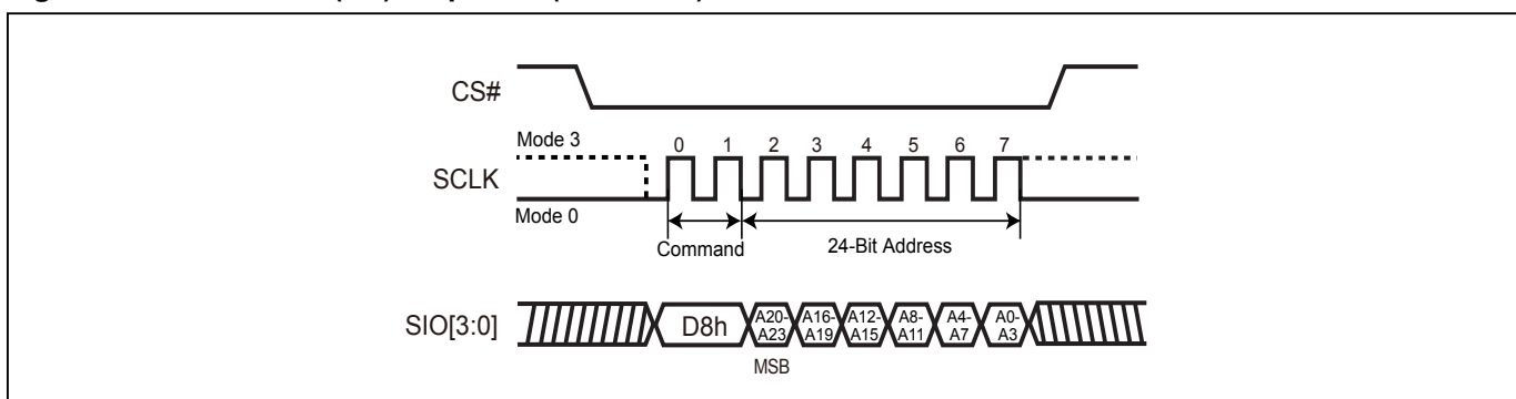
Figure 59. Block Erase (BE) Sequence (QPI Mode)
