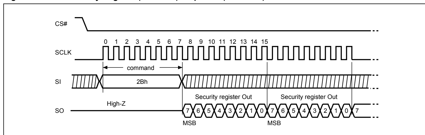
Figure 79. Read Security Register (RDSCUR) Sequence (SPI Mode)
