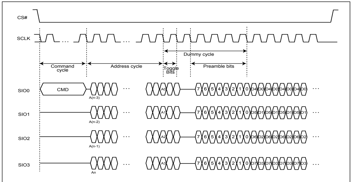
Figure 50. DTR4IO (6DC)
