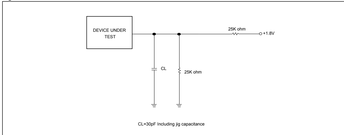
Figure 104. OUTPUT LOADING
