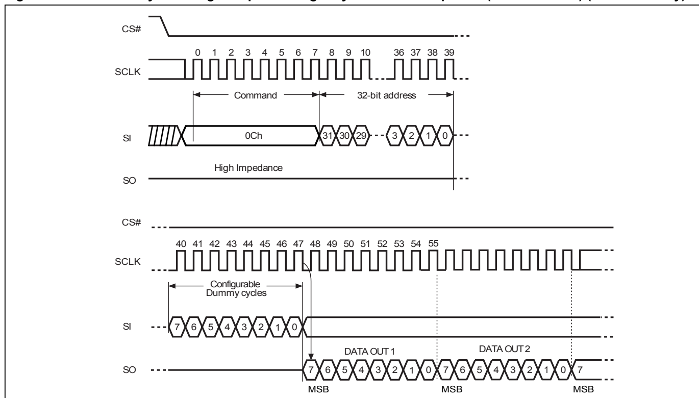
Figure 50. Read Data Bytes at Higher Speed using 4 Byte Address Sequence (FASTREAD4B) (SPI Mode only)
