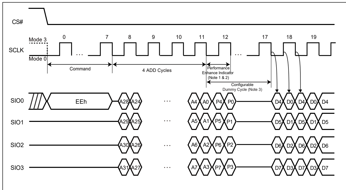
Figure 53. Fast Quad I/O DT Read (4DTRD4B) Sequence (SPI Mode only)
