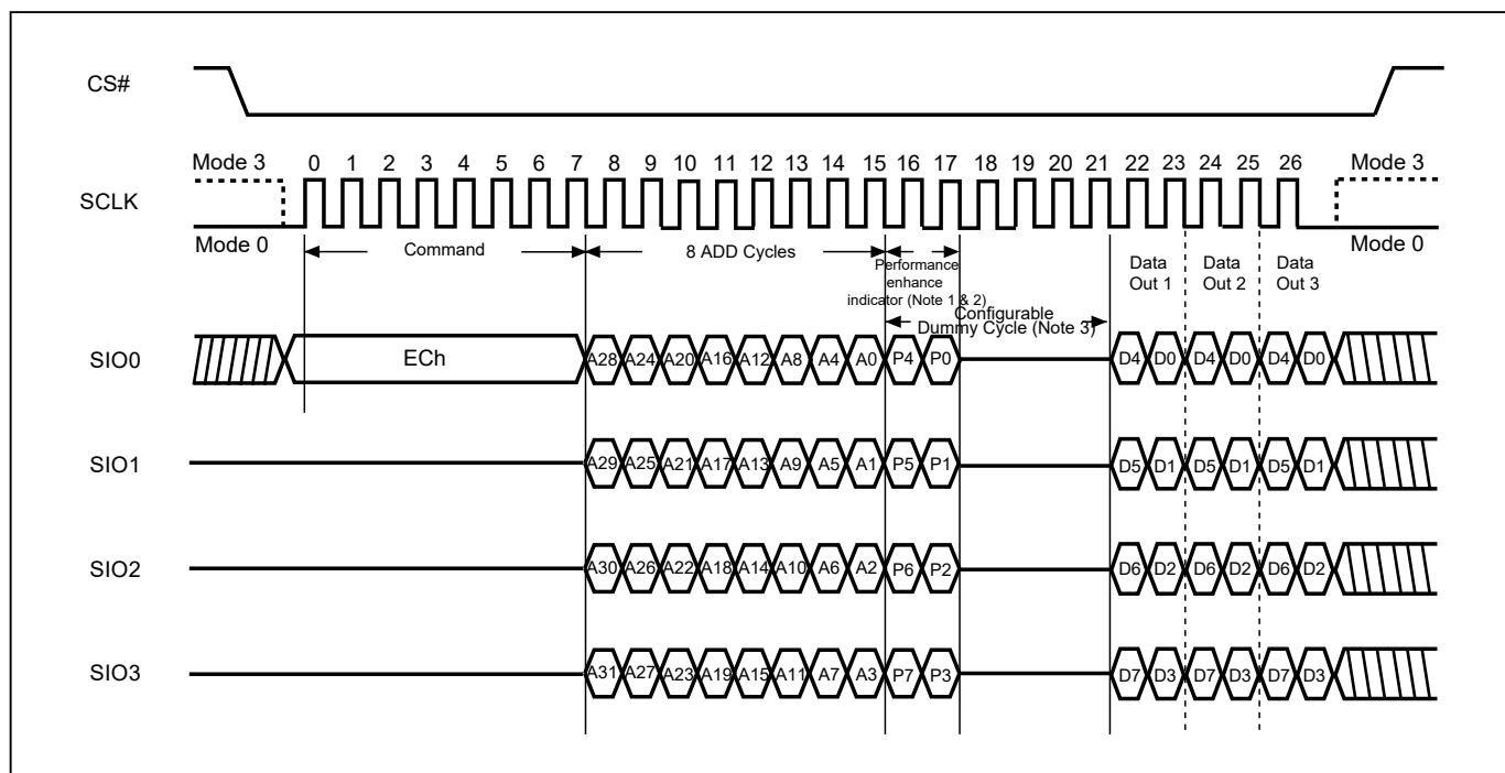
Figure 52. 4 I/O Fast Read using 4 Byte Address sequence (4READ4B) (SPI Mode only)
