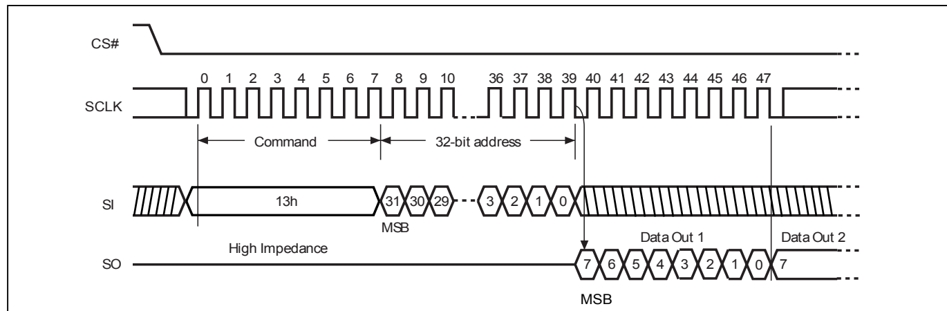
Figure 49. Read Data Bytes using 4 Byte Address Sequence (READ4B) (SPI Mode only)
