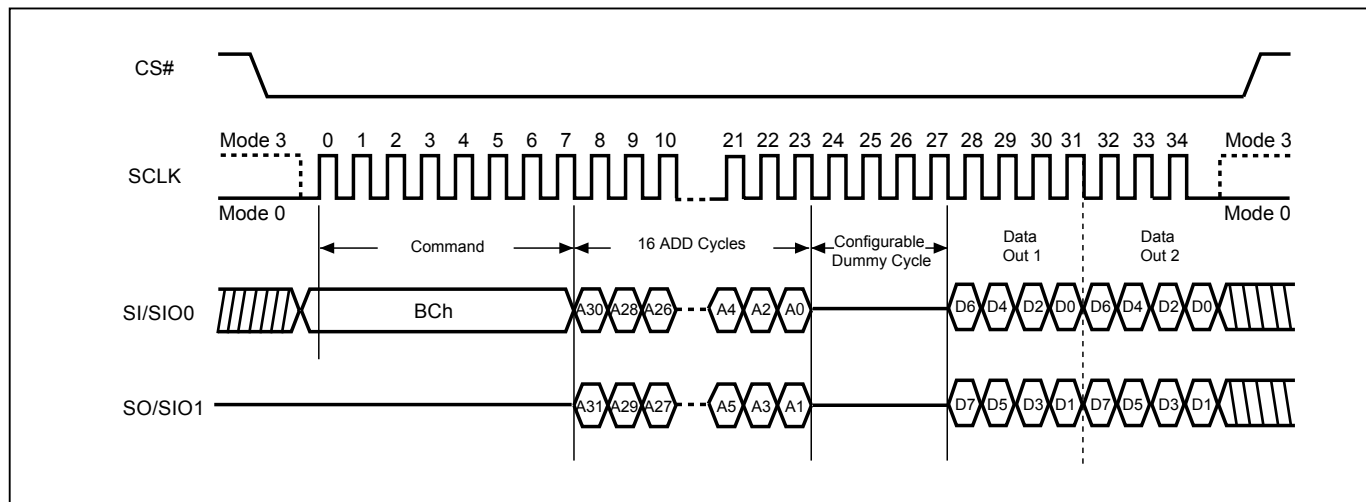
Figure 51. 2 x I/O Fast Read using 4 Byte Address Sequence (2READ4B) (SPI Mode only)
