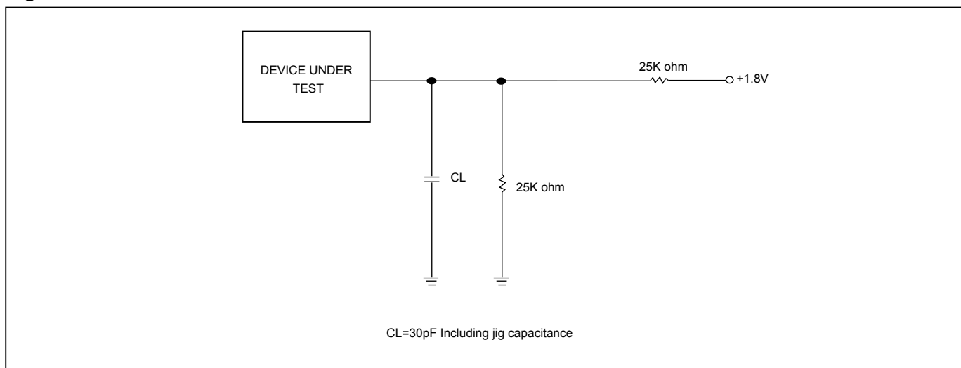
Figure 80. OUTPUT LOADING
