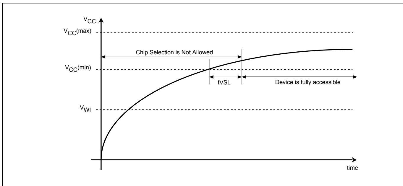
Figure 84. Power-up Timing
