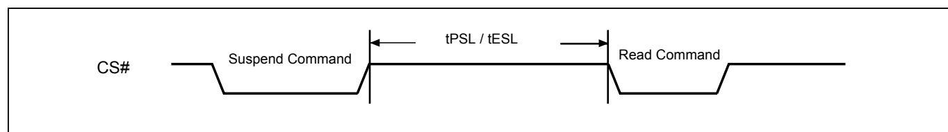
Figure 110. Suspend to Read Latency
