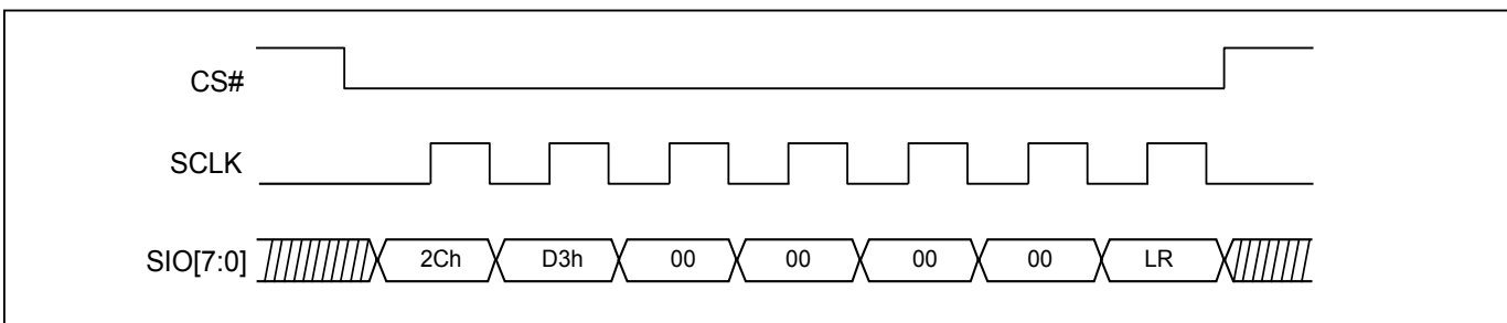
Figure 84. Write Lock Register (WRLR) Sequence (STR-OPI Mode)
