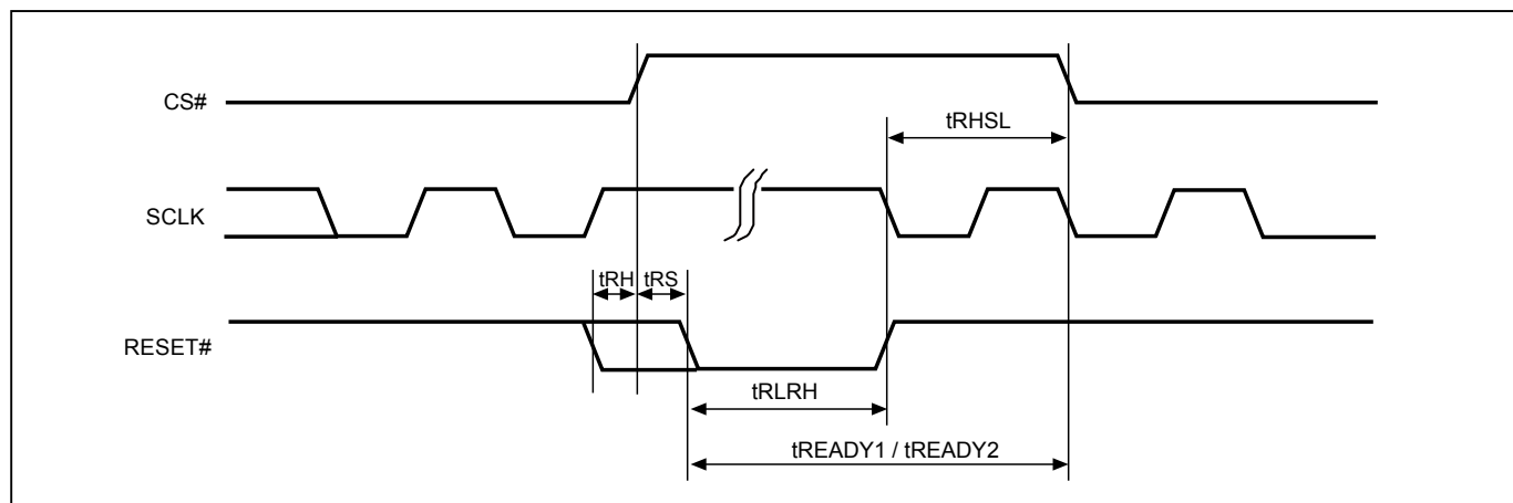
Figure 129. RESET Timing
