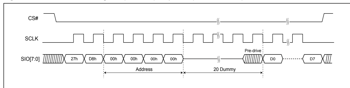
Figure 102. Read Password Register (RDPASS) Sequence (STR-OPI Mode)
