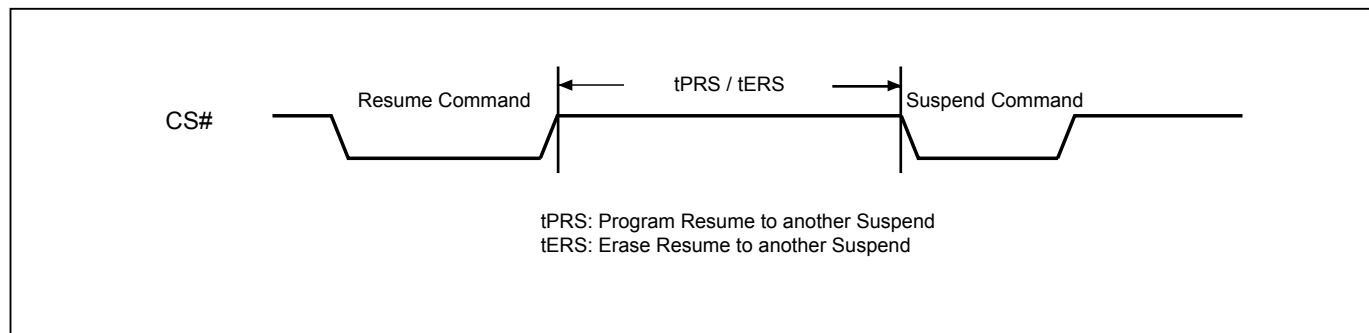
Figure 97. Resume to Suspend Latency
