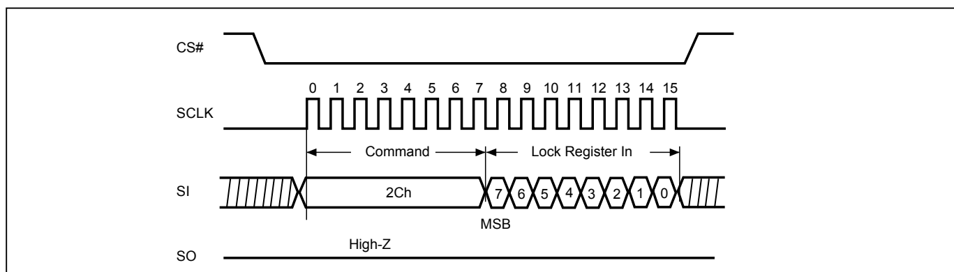
Figure 83. Write Lock Register (WRLR) Sequence
