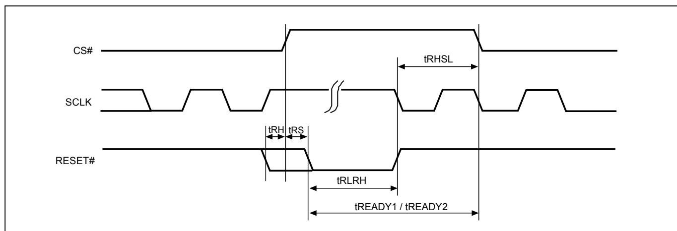
Figure 104. RESET Timing
