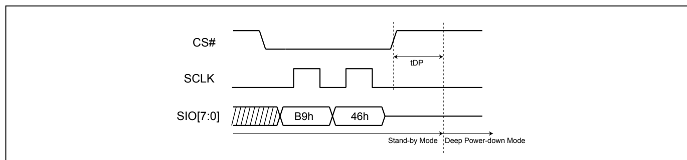
Figure 74. Deep Power-down (DP) Sequence (STR-OPI Mode)
