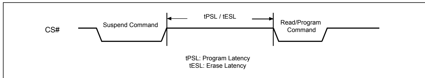
Figure 95. Suspend to Read/Program Latency
