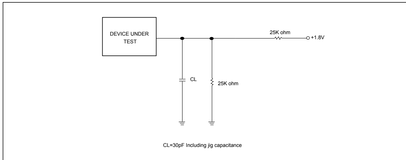
Figure 108. OUTPUT LOADING
