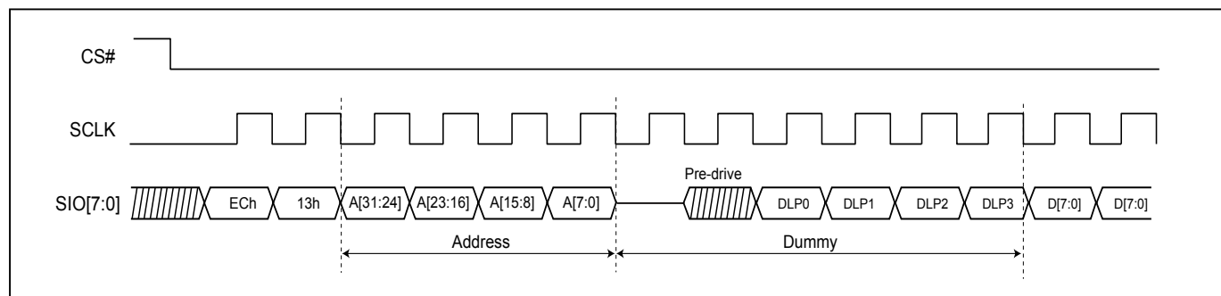
Figure 44. Preamble Bit data pattern Output Sequence (STR-OPI Mode)
