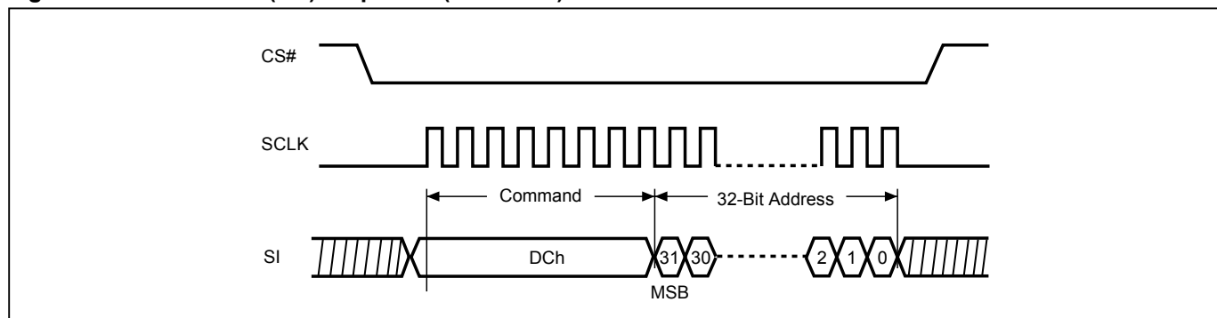
Figure 64. Block Erase (BE) Sequence (SPI Mode)
