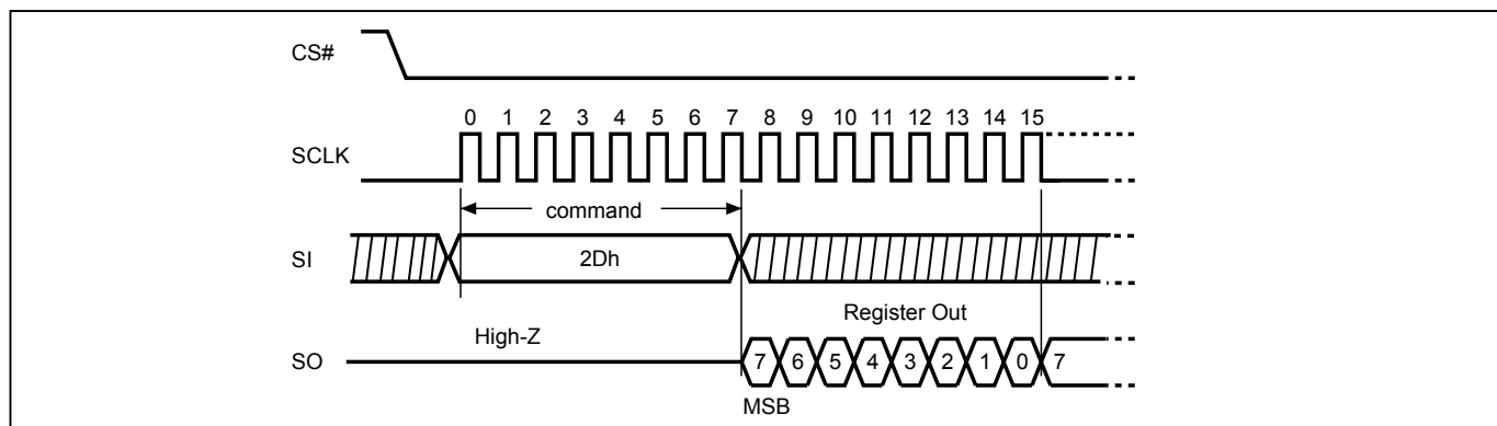
Figure 80. Read Lock Register (RDLR) Sequence
