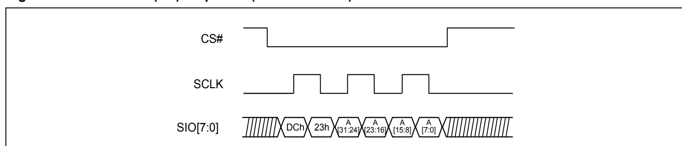
Figure 66. Block Erase (BE) Sequence (DTR-OPI Mode)
