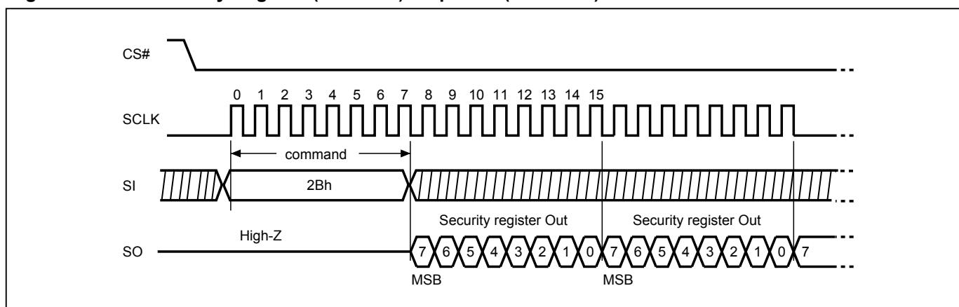
Figure 34. Read Security Register (RDSCUR) Sequence (SPI Mode)
