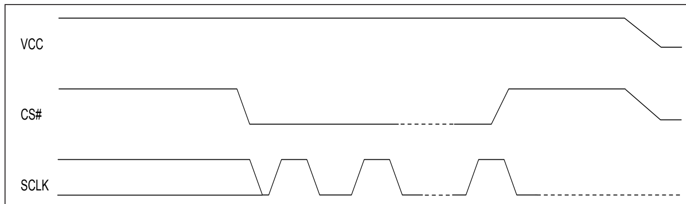
Figure 28. Power-Down Sequence
