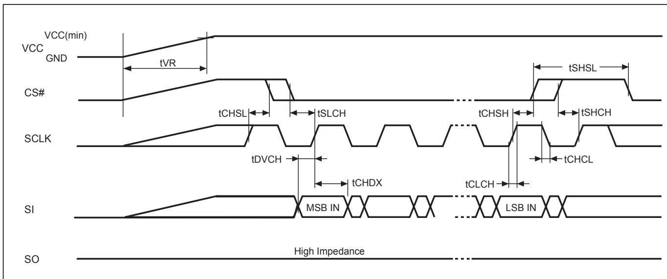
Figure 27. AC Timing at Device Power-Up
