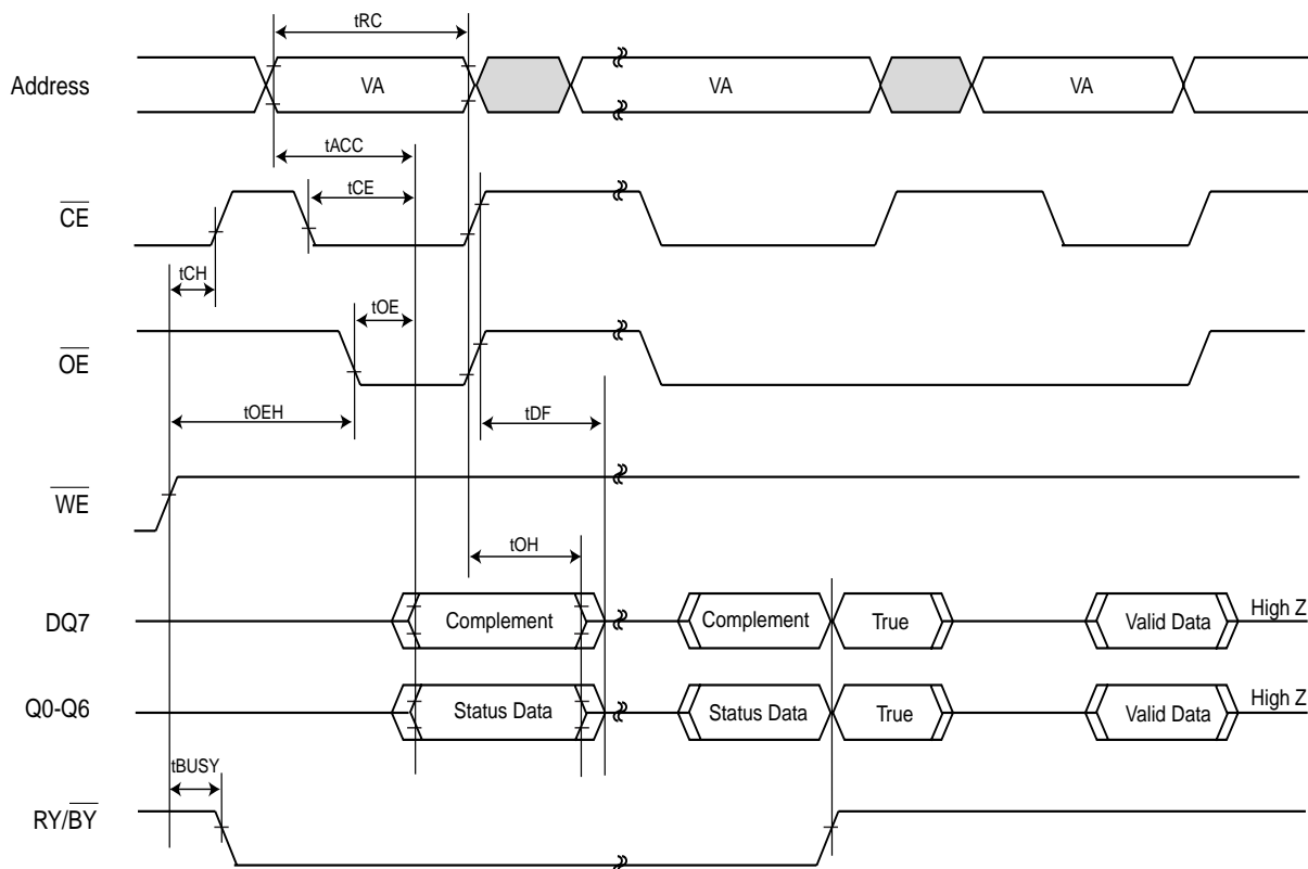
Figure 18. Data Polling Timings (During Automatic Algorithms)
