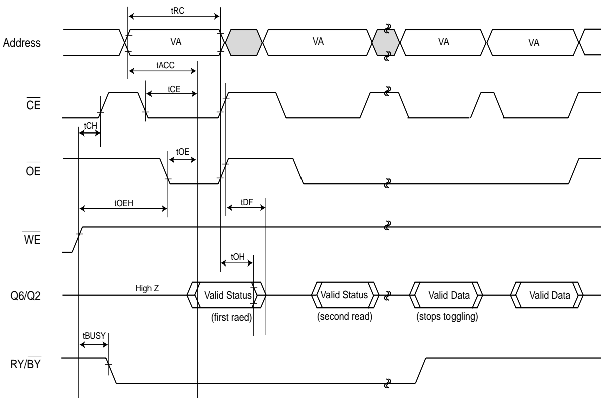
Figure 19. Toggle Bit Timings (During Automatic Algorithms)
