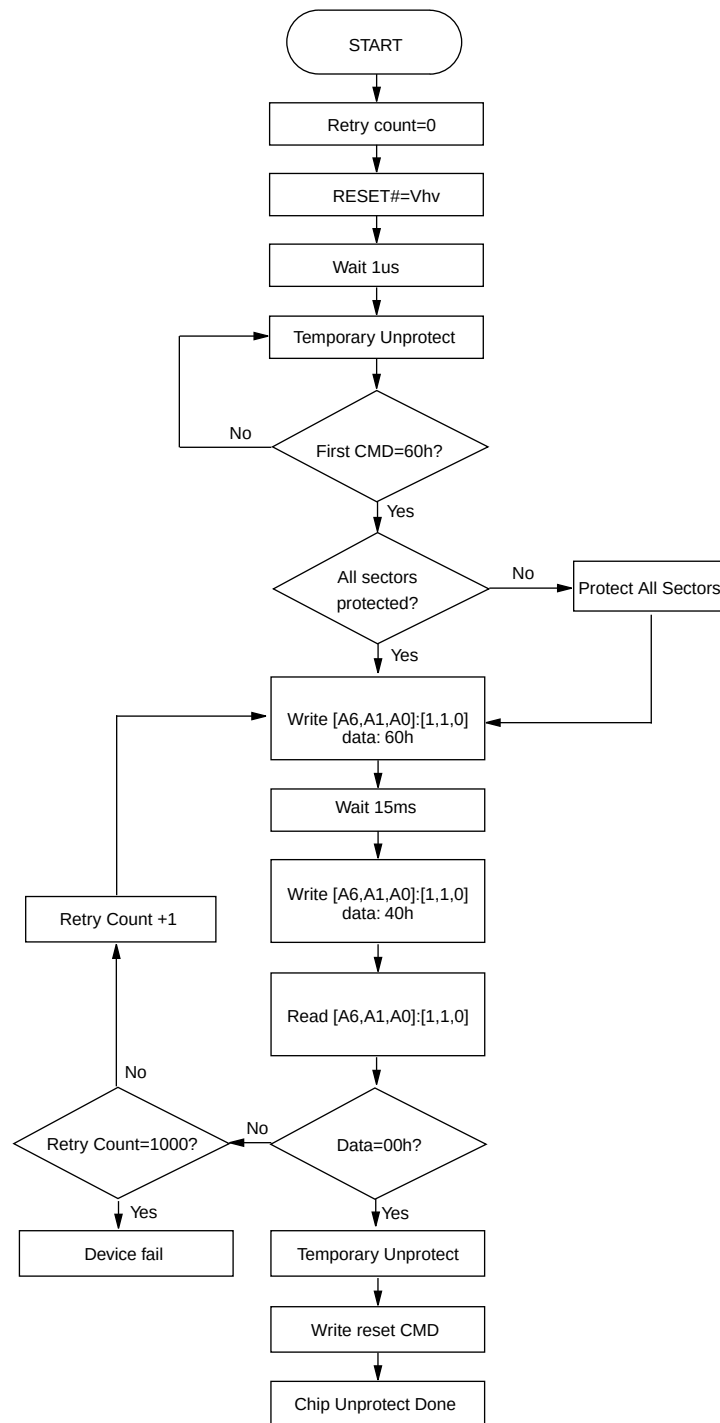
Figure 14-2. CHIP UNPROTECT ALGORITHMS WITH RESET#=Vhv
