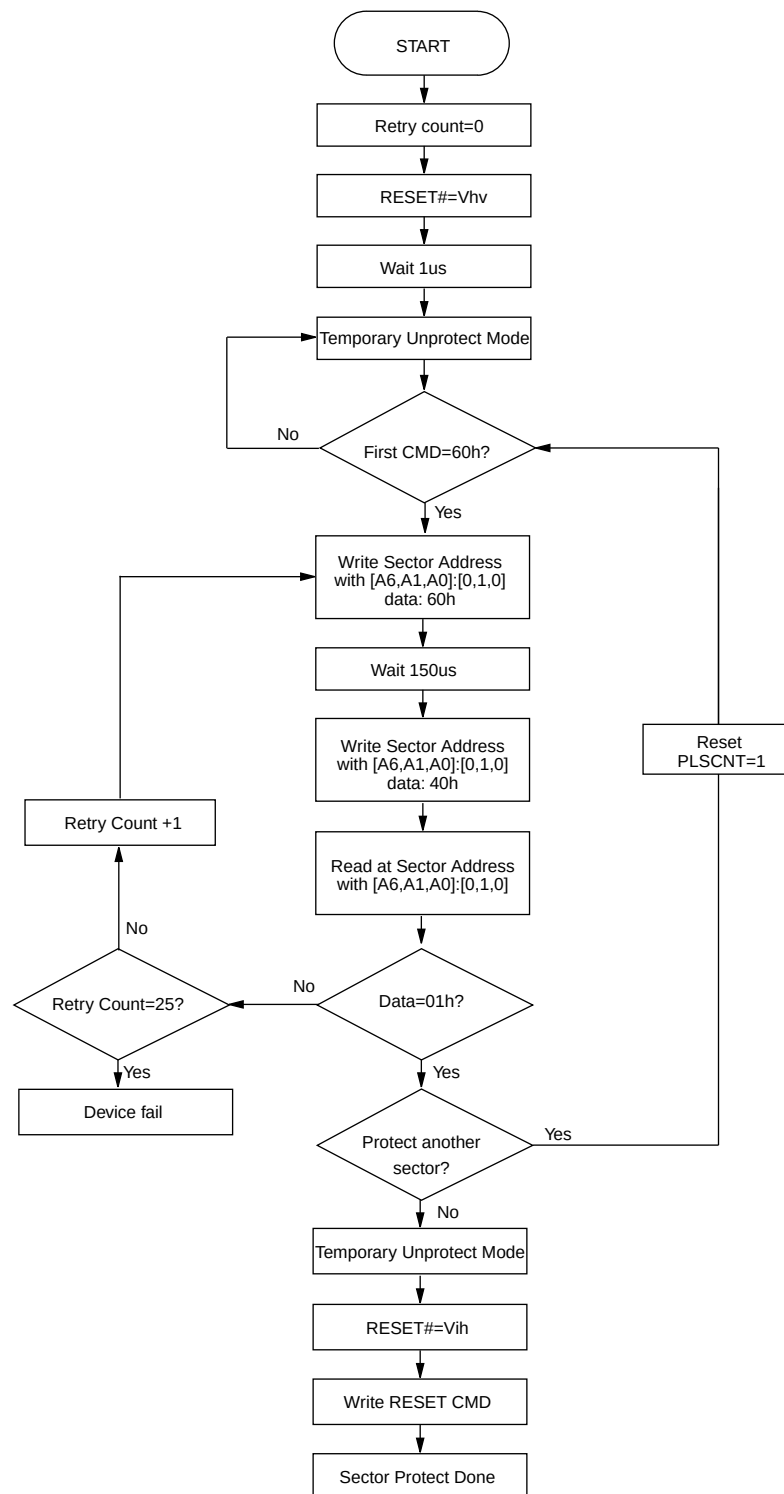
Figure 14-1. IN-SYSTEM SECTOR GROUP PROTECT WITH RESET# = V h v
