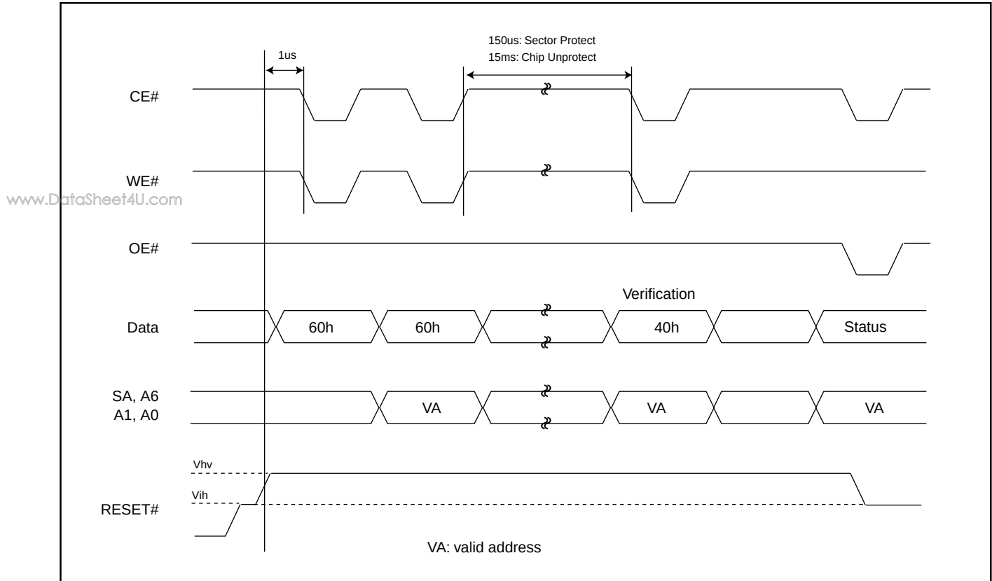
Figure 13. SECTOR GROUP PROTECT/CHIP UNPROTECT WAVEFORM (RESET# Control)
