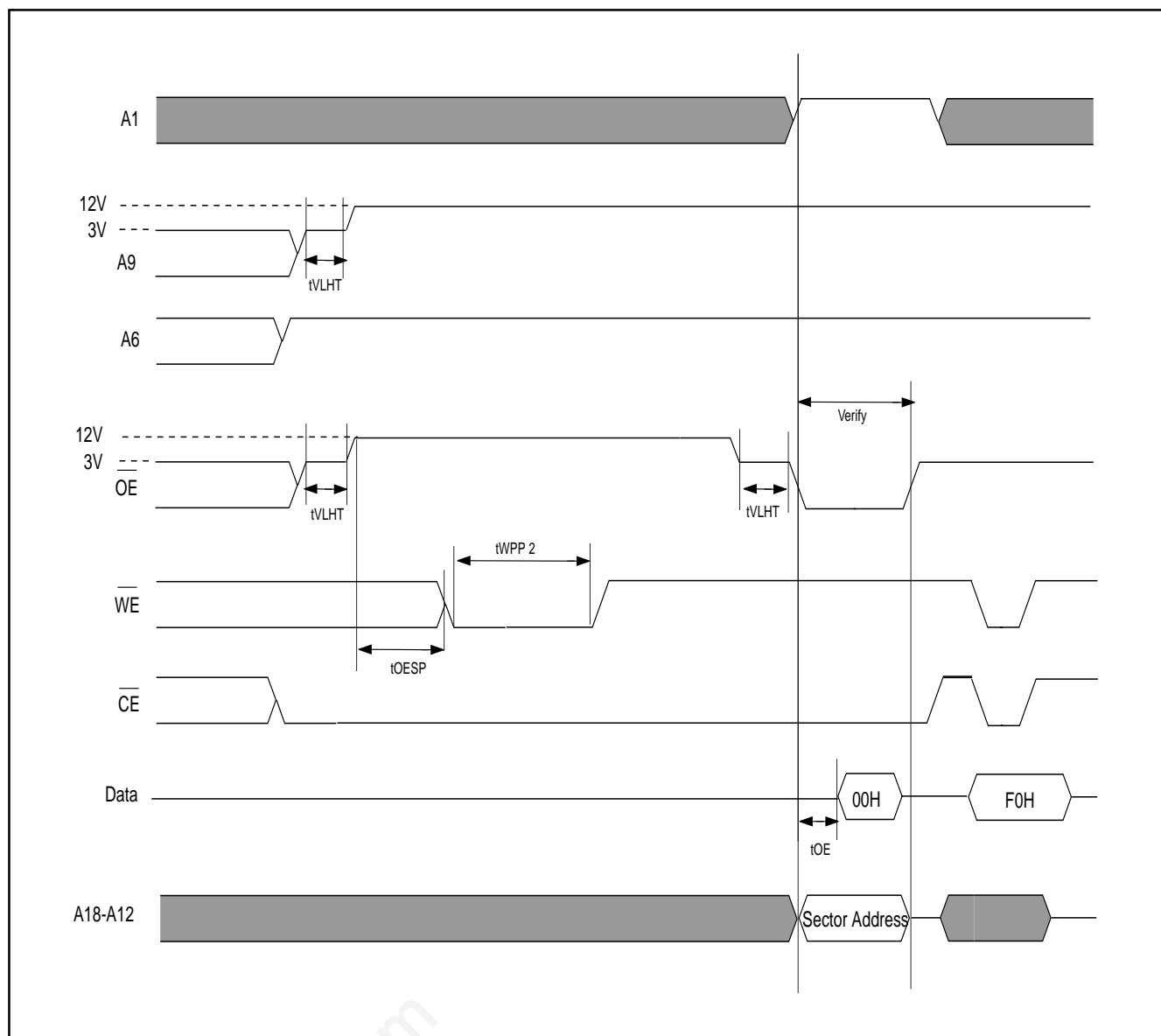
Figure 18. TIMING WAVEFORM FOR CHIP UNPROTECTION (A9, \overline{OE} Control)
