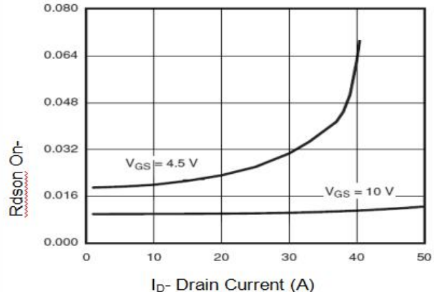
Figure 6 Drain-Source On-Resistance
