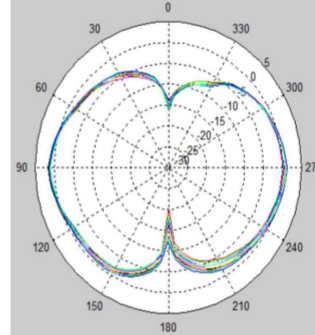
2.4G vertical pattern
