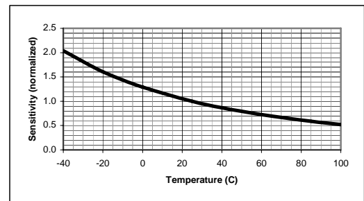
Figure 1: Thermal Accelerometer Sensitivity
