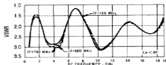
R-Port VSWR vs. Frequency
