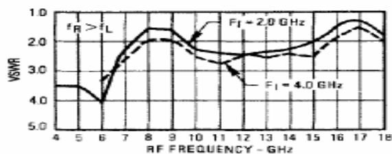
R-Port VSWR L_o @ +21 dBm
