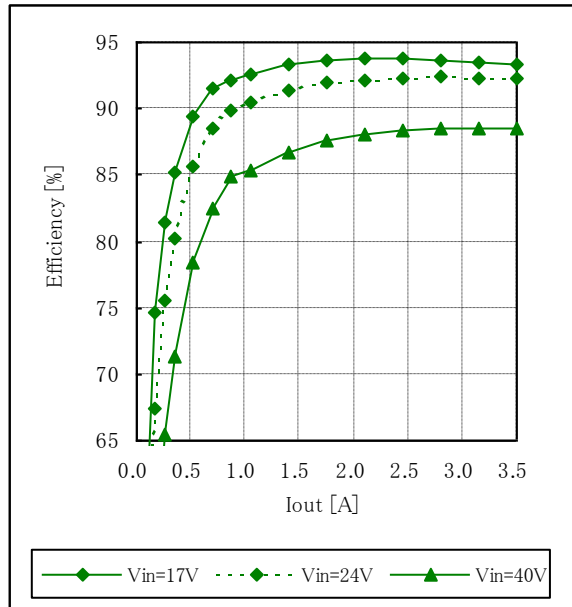
Fig.12-1-2. Efficiency vs. Output Current
