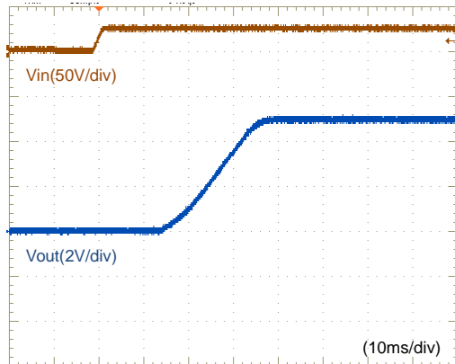
Fig.12-2-1. Start-up Waveform ( I_o=0A )
