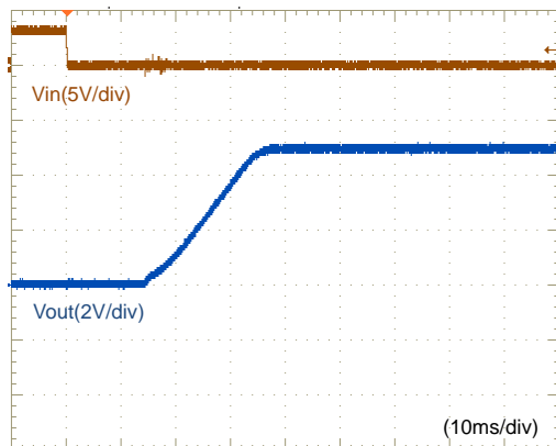
Fig.12-2-3. Start-up Waveform ( I_o=0A )
