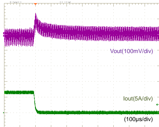
Fig.12-2-18. Load Transient Response ( I_o= 6A \rightarrow 0 )
