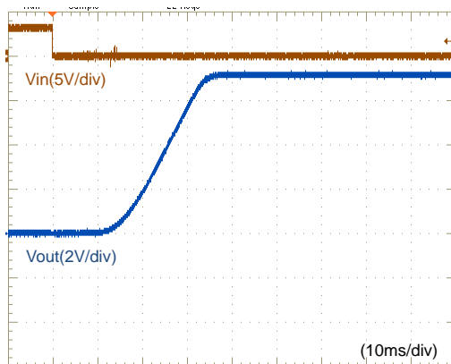
Fig.12-2-21. Start-up Waveform ( I_o=0A )
