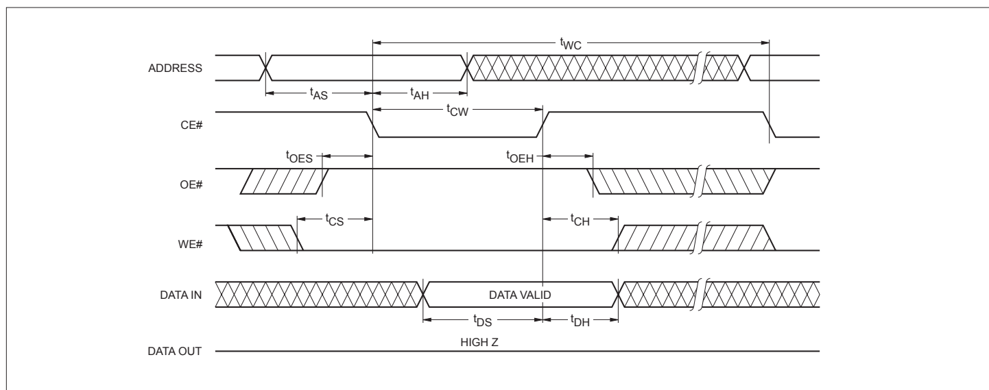
Figure 16 - CE# Controlled Write Cycle
