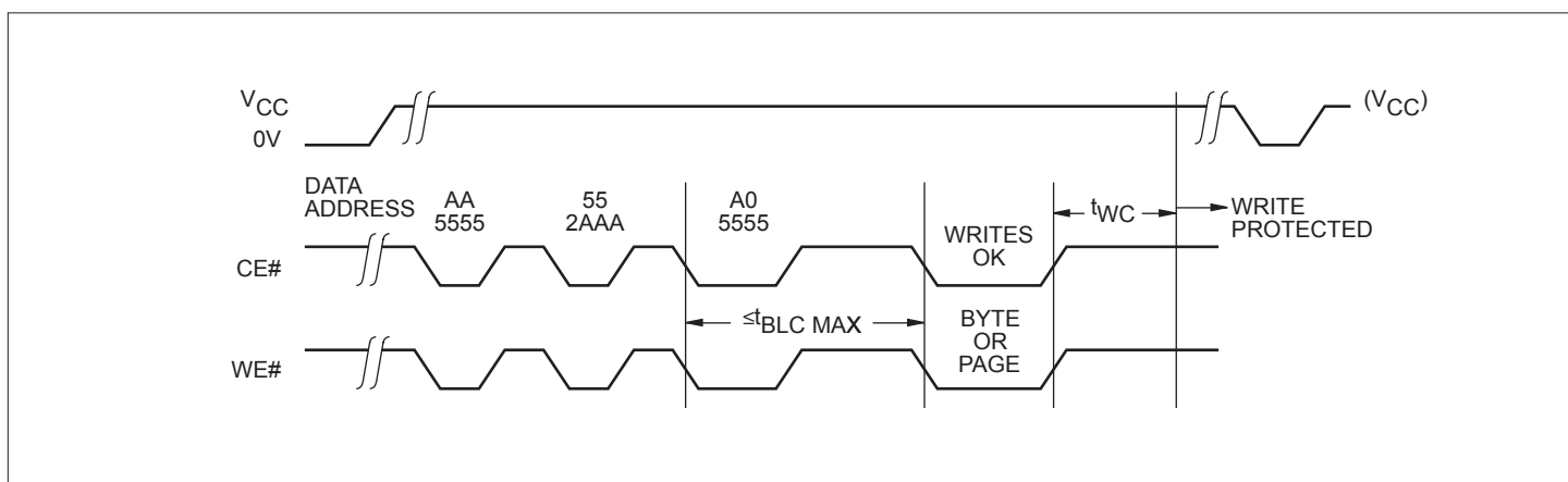
Figure 8 - Timing Sequence - Byte or Page Write
