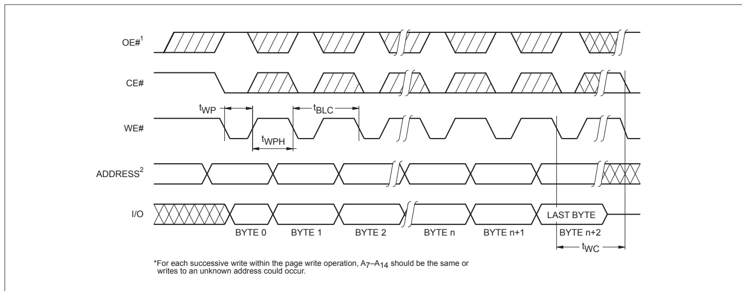
Figure 17 - Page Write Cycle
