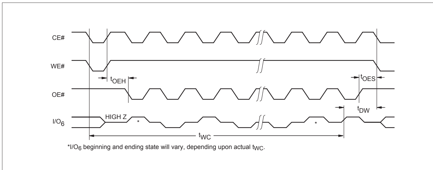
Figure 19 - Toggle Bit Timing Diagram 1
