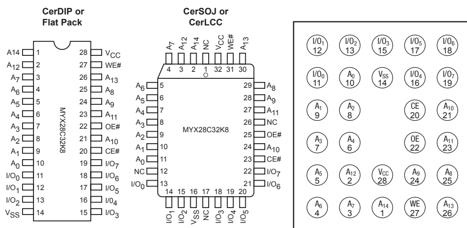
Figure 1 - Pin Configuration
