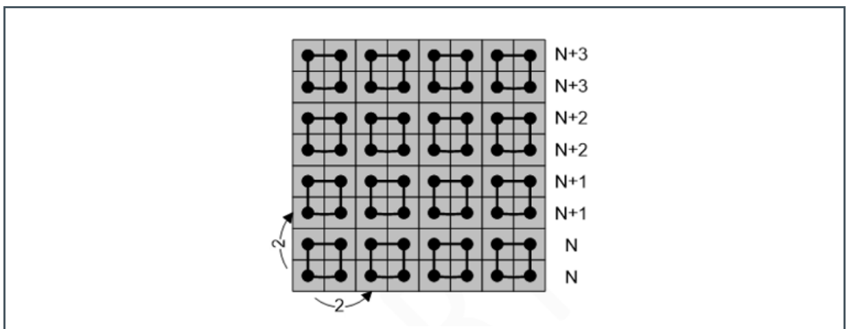
Figure 55: Binning Mode
