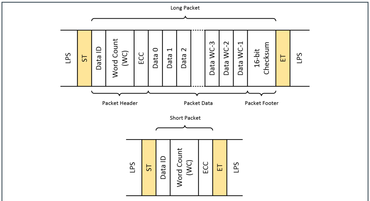
Figure 30: MIPI Long & Short Packet Structure Diagrams
