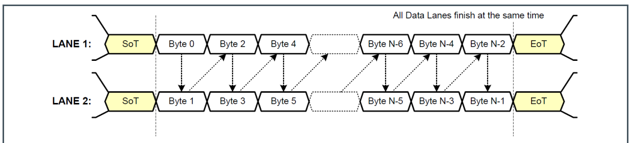
Figure 31: MIPI 1/2/4-Lane Data Package Transmission
