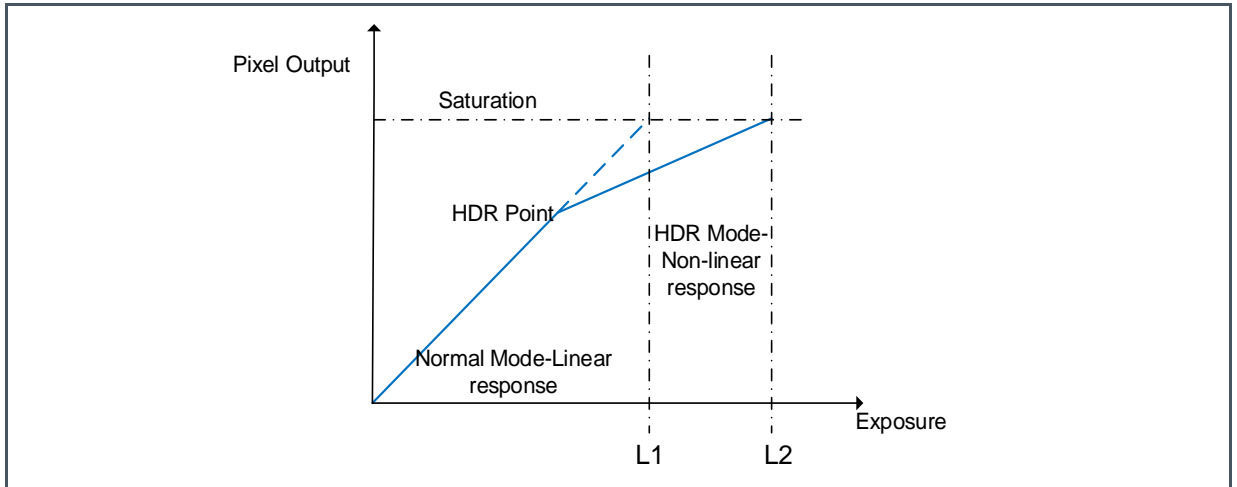
Figure 40: Normal and HDR Modes
