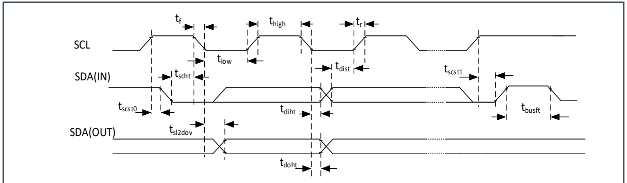
Figure 24: I 2 C Interface Timing
