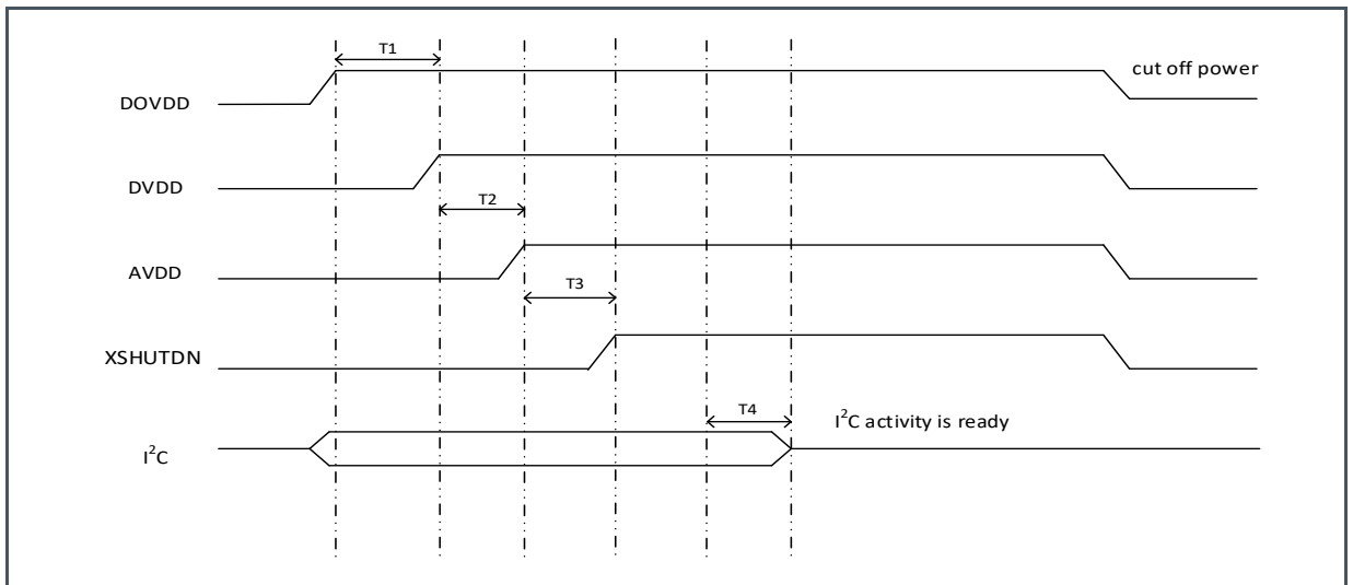
Figure 18: Power-Up Sequence
