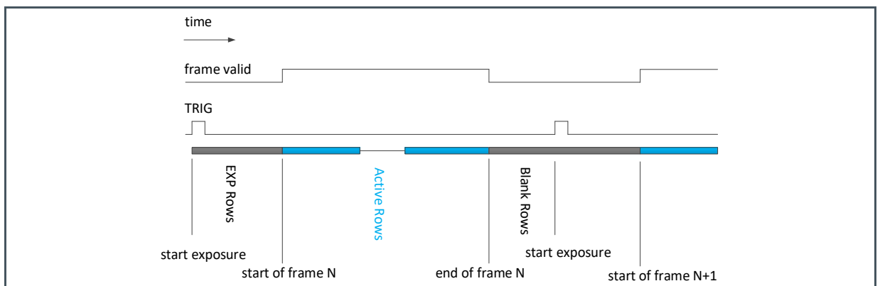
Figure 36: External Triggering Global Shutter Mode Timing Diagram
