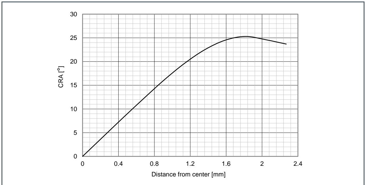
Figure 17: CRA Versus Distance from Center
