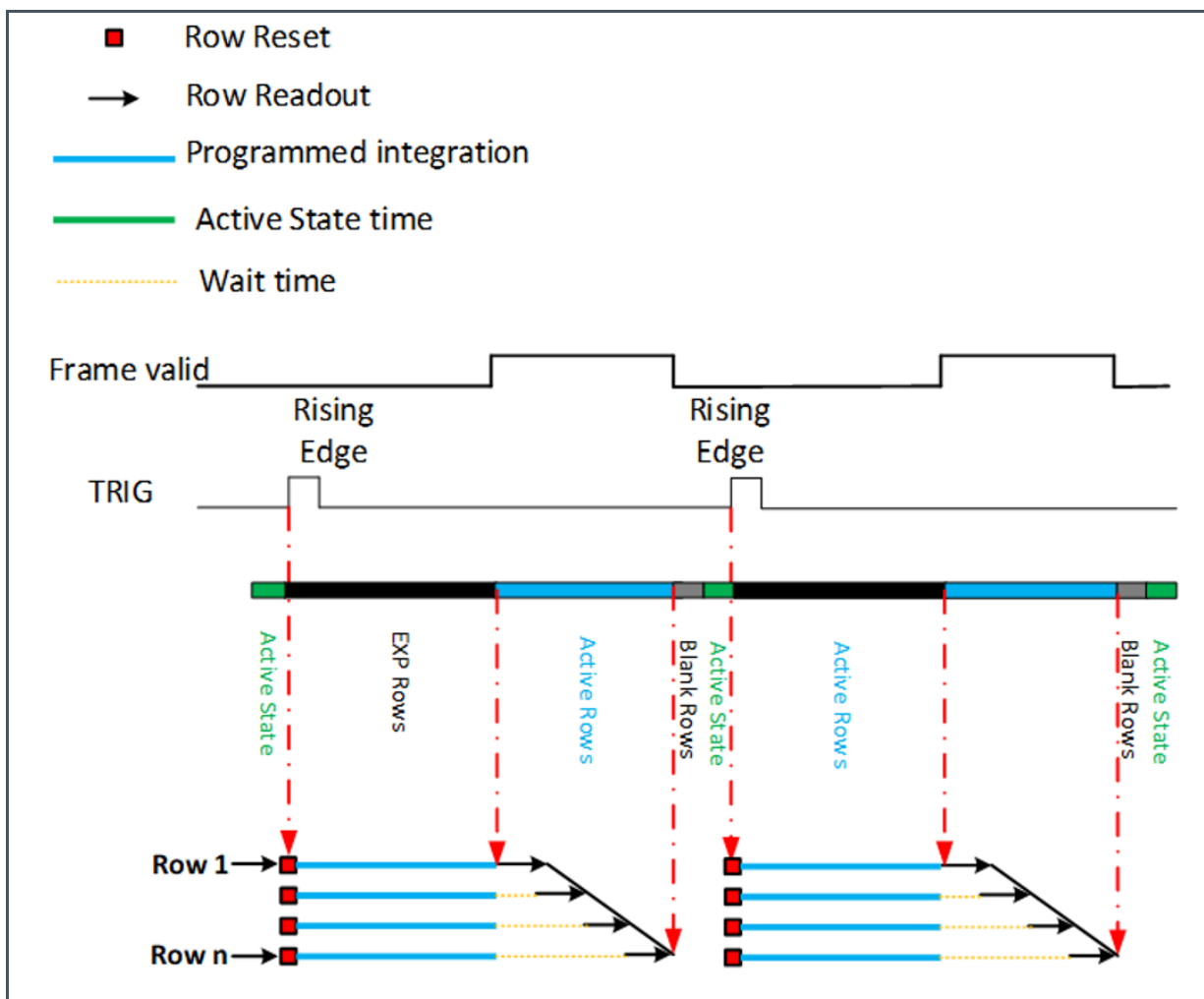
Figure 39: External Trigger Timing
