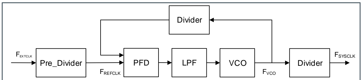
Figure 34: PLL Block Diagram
