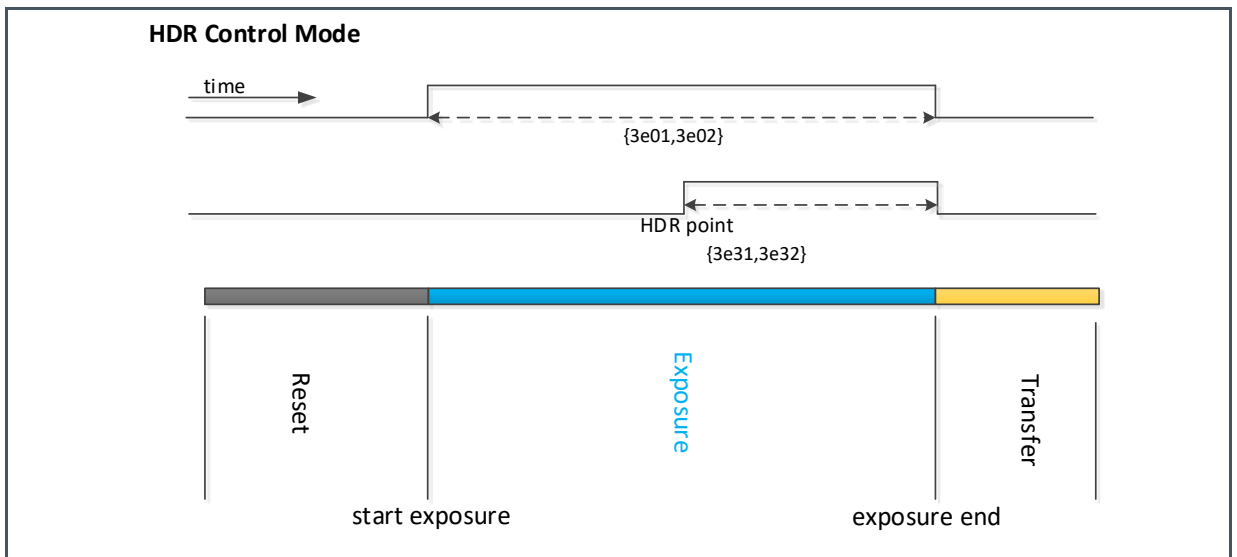
Figure 41: HDR Mode Timing
