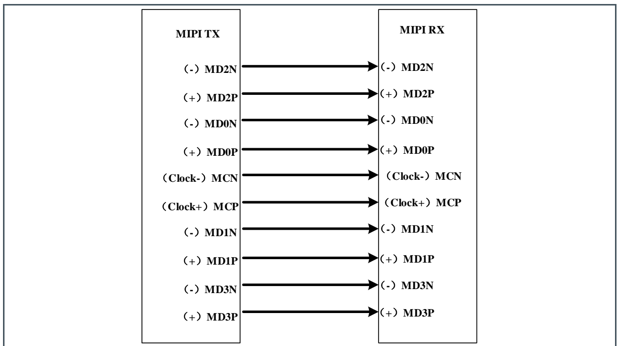
Figure 27: MIPI Interface
