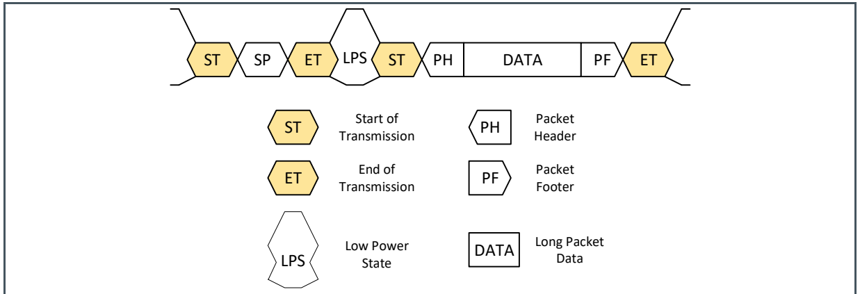
Figure 28: MIPI Low Level Data Packet
