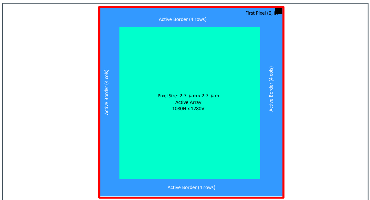
Figure 50: Mira130 Pixel Array
