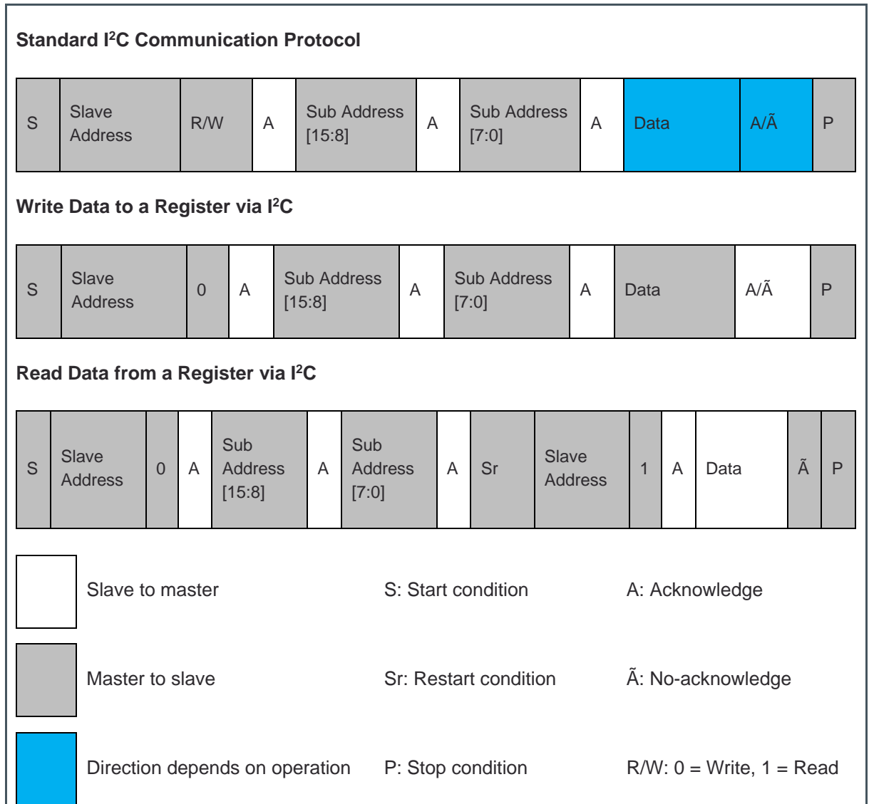
Figure 23: I 2 C Bus Device Address Control Example
