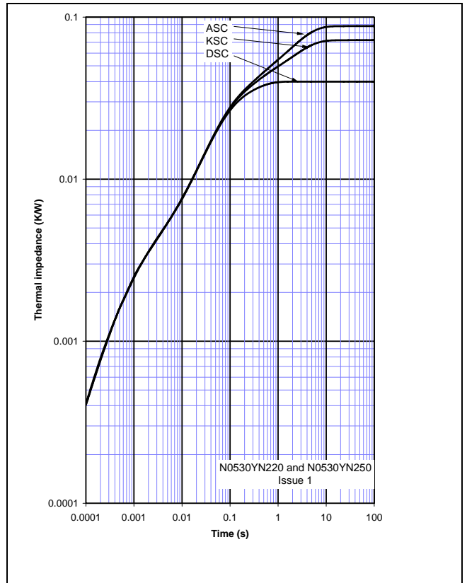
Figure 2 – Transient thermal impedance junction to case
