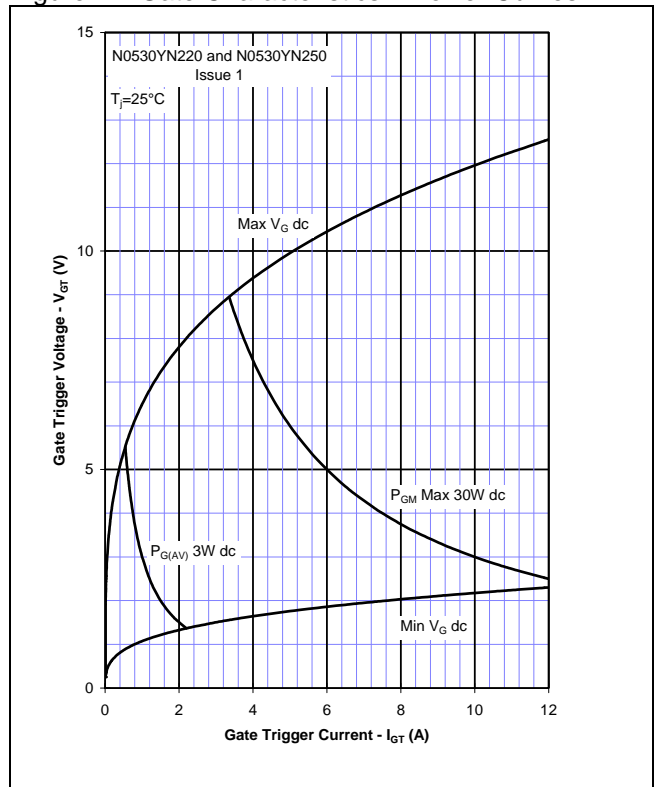
Figure 4 – Gate Characteristics – Power Curves
