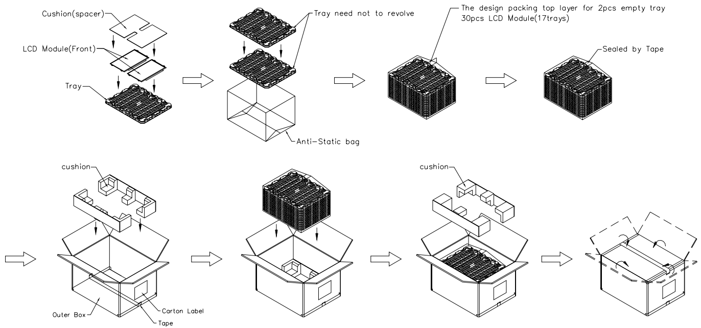
Figure. 10-1 Packing method
