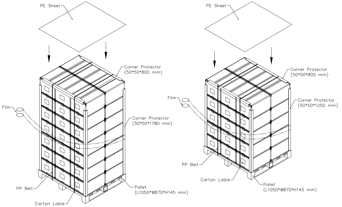
Figure. 10-2 Packing method
