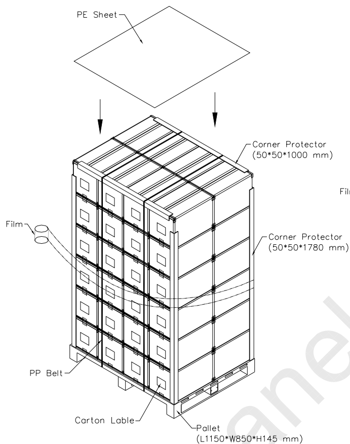
Figure. 10-2 Packing method
