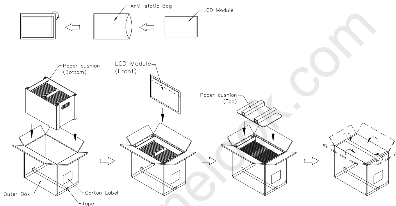
Figure. 10-1 Packing method
