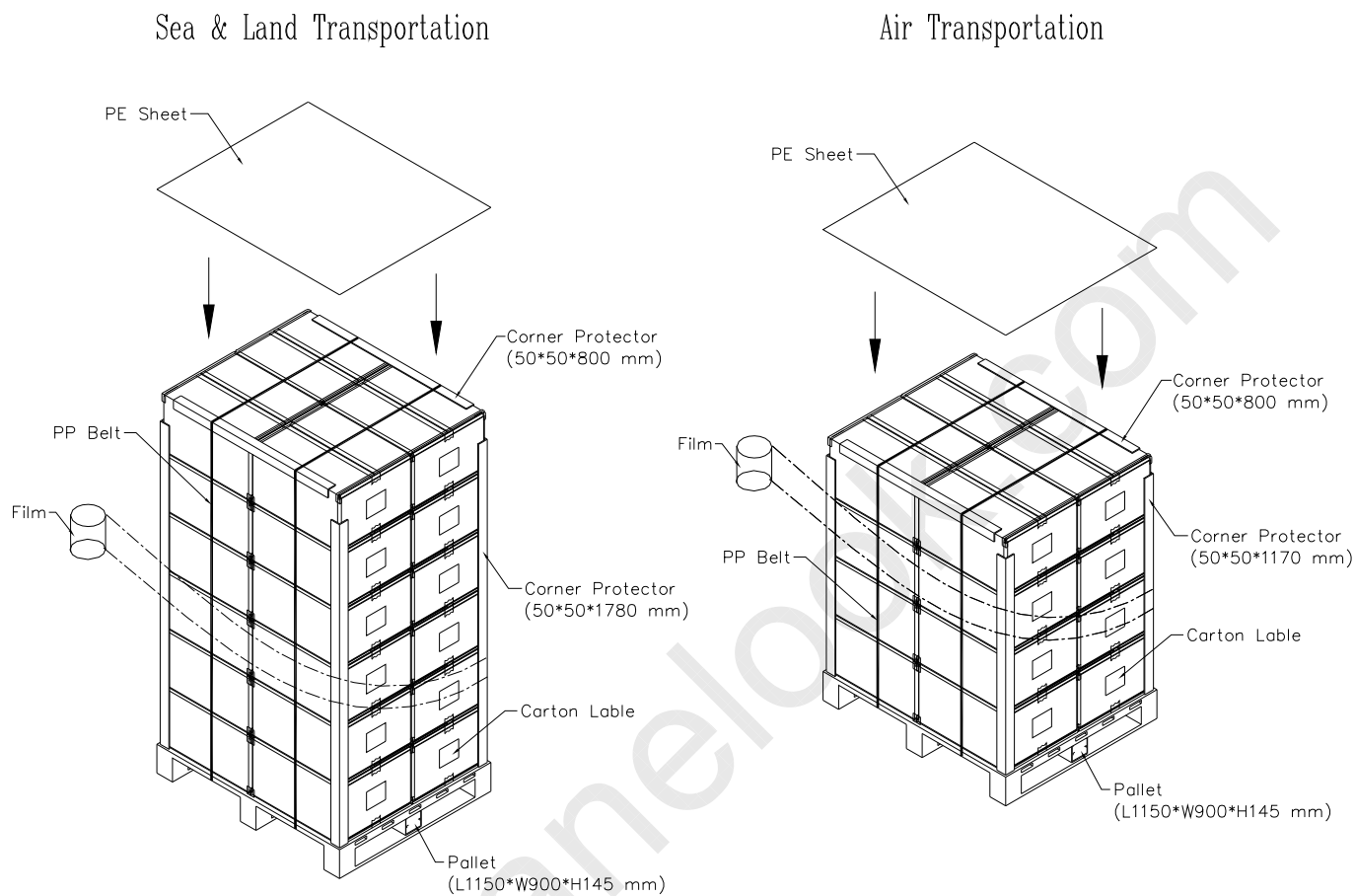
Figure. 10-2 Packing method
