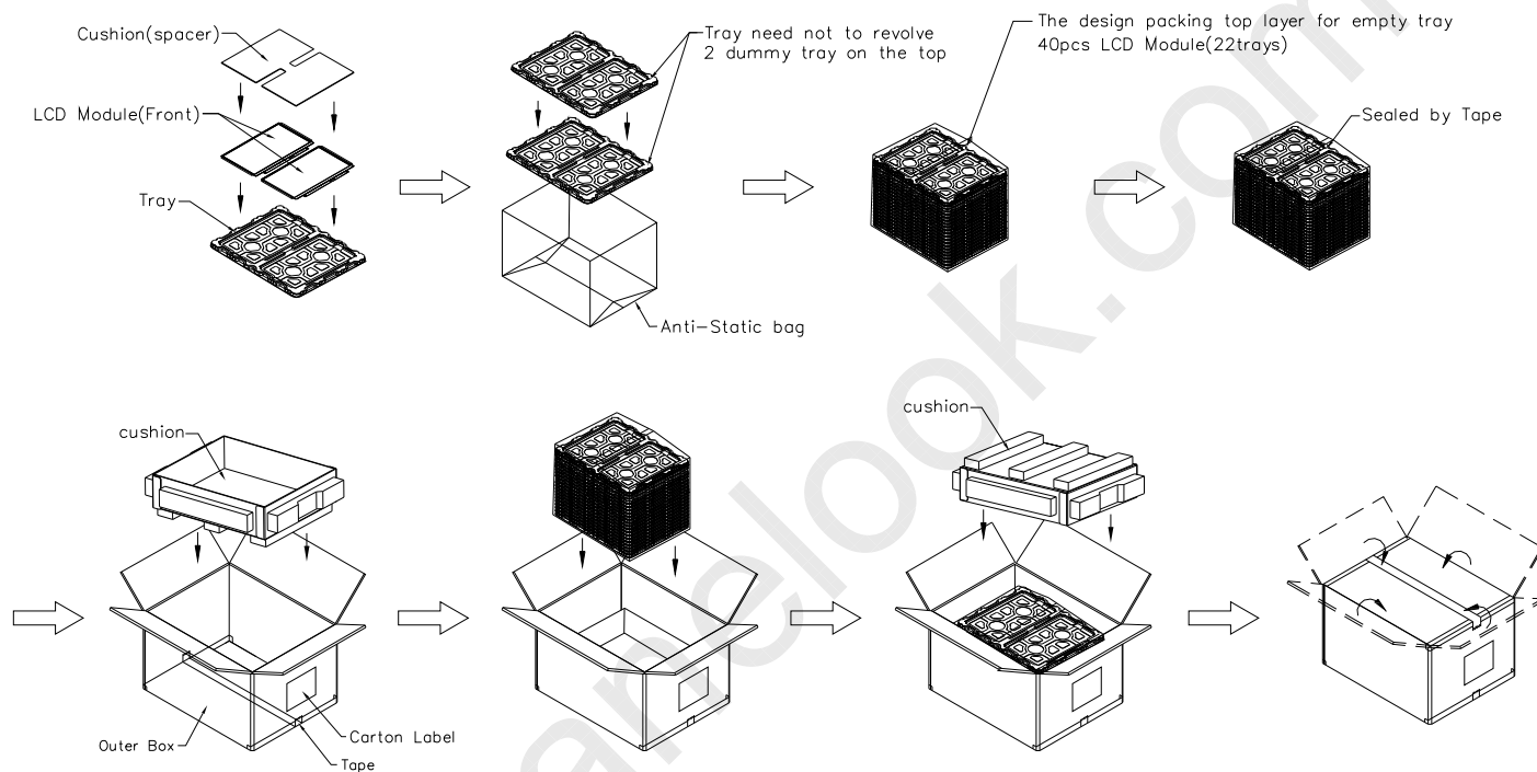
Figure. 10-1 Packing method
