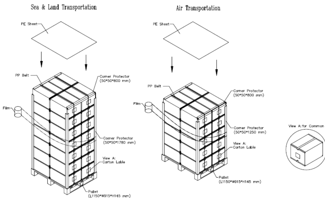
Figure. 7-2 Packing method
