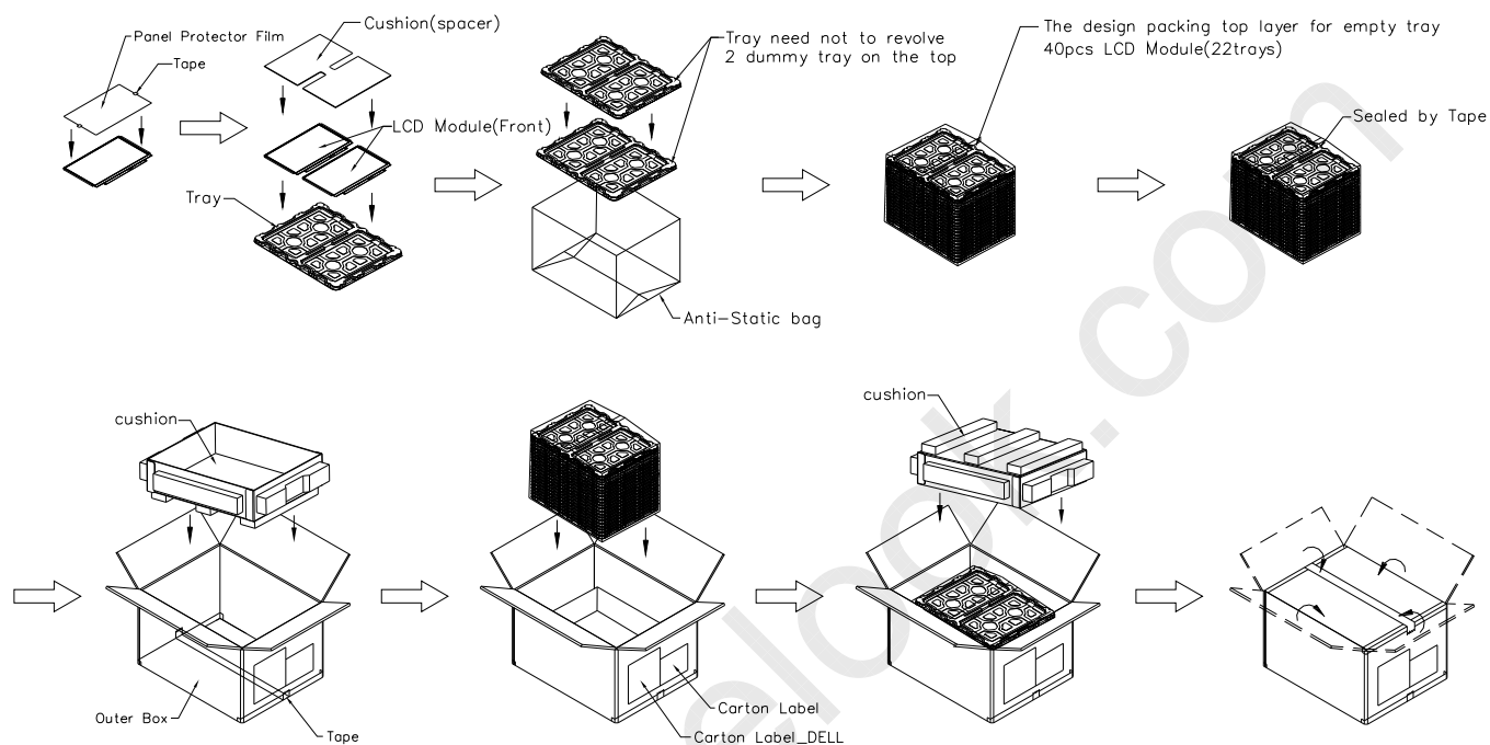
Figure. 7-3 Packing method
