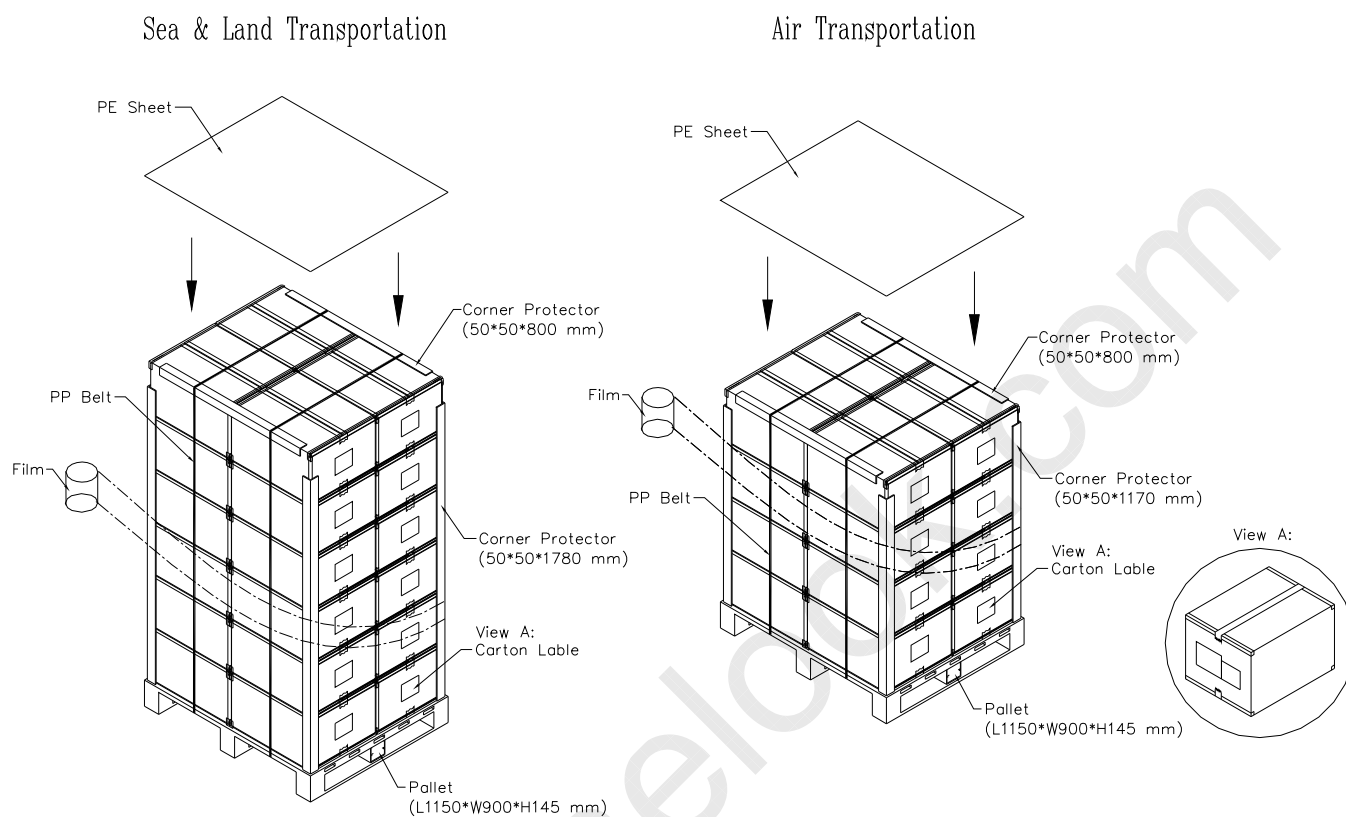
Figure. 7-4 Packing method
