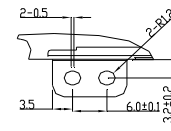
DETAIL D SCALE 2:1
