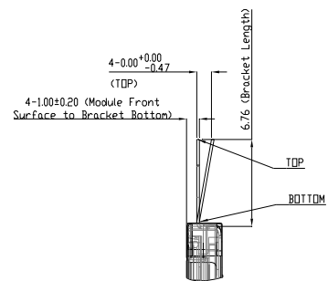
DETAIL E SCALE 5:1
