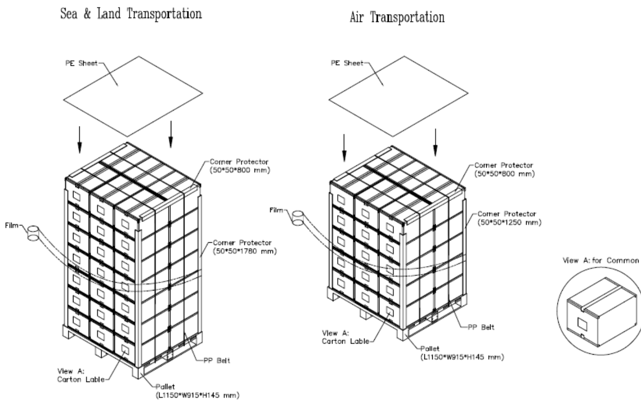
Figure. 7-2 Packing method
