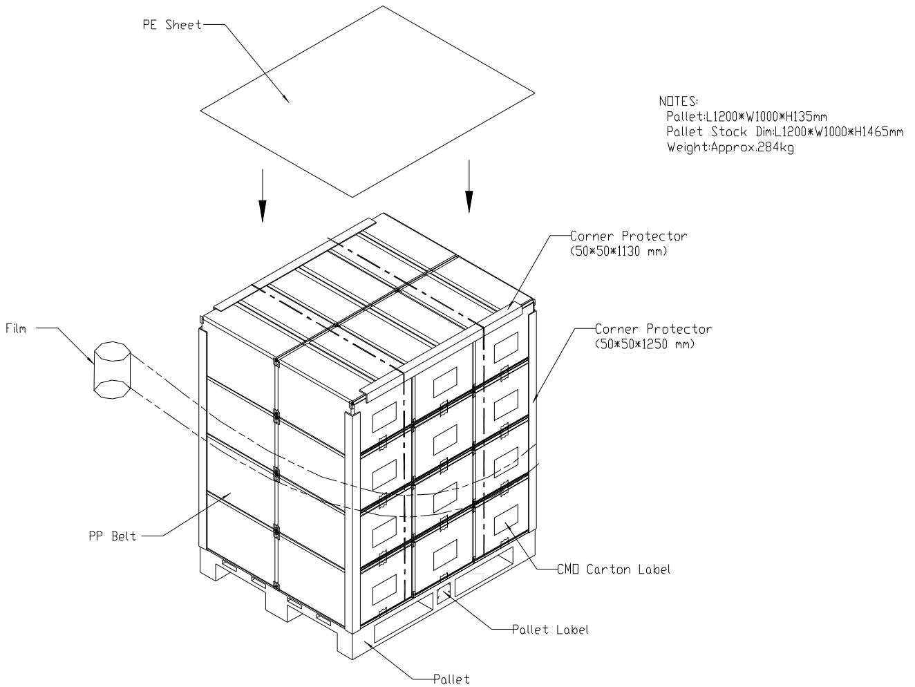
Figure. 10-3 Packing method
