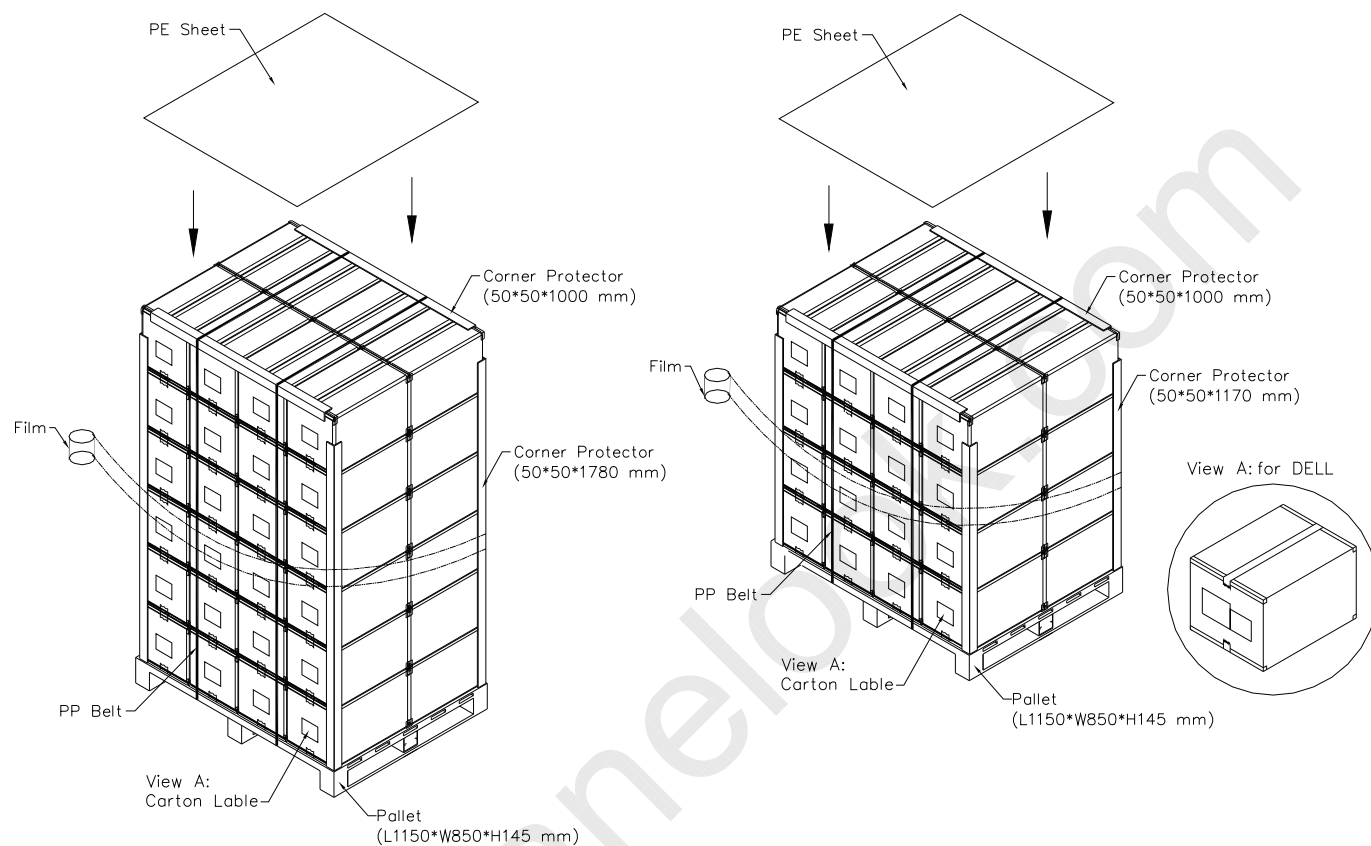
Figure. 11-2 Packing method
