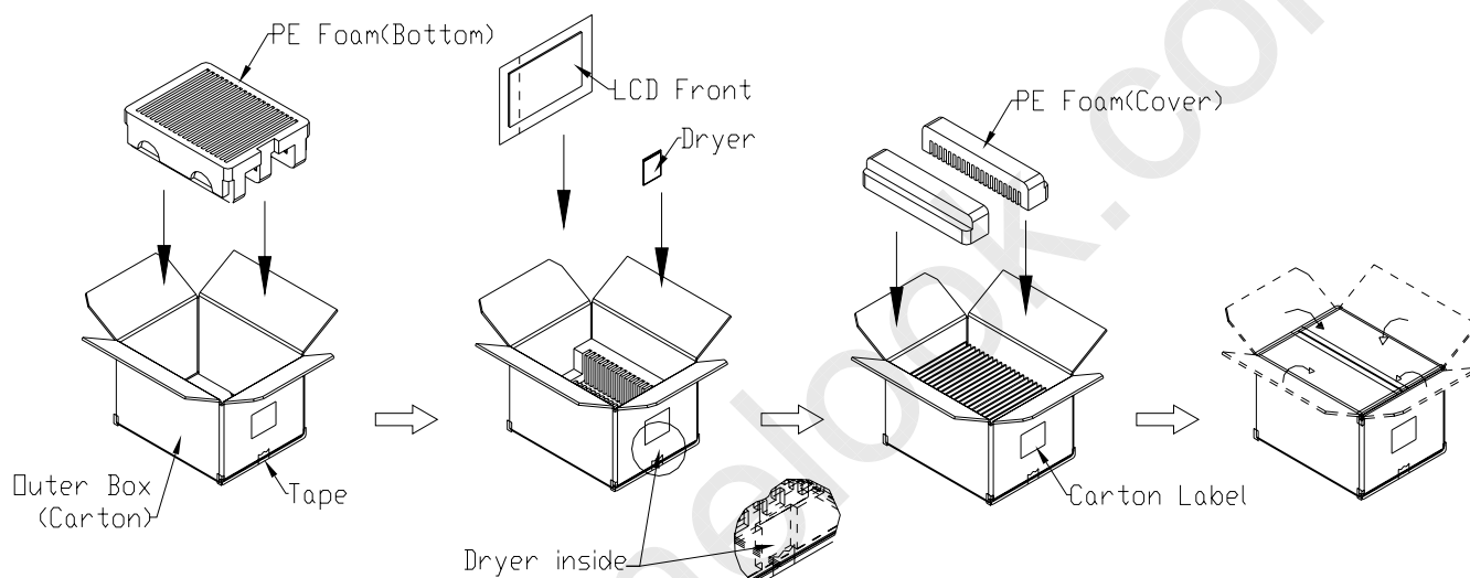
Figure. 10-1 Packing method
