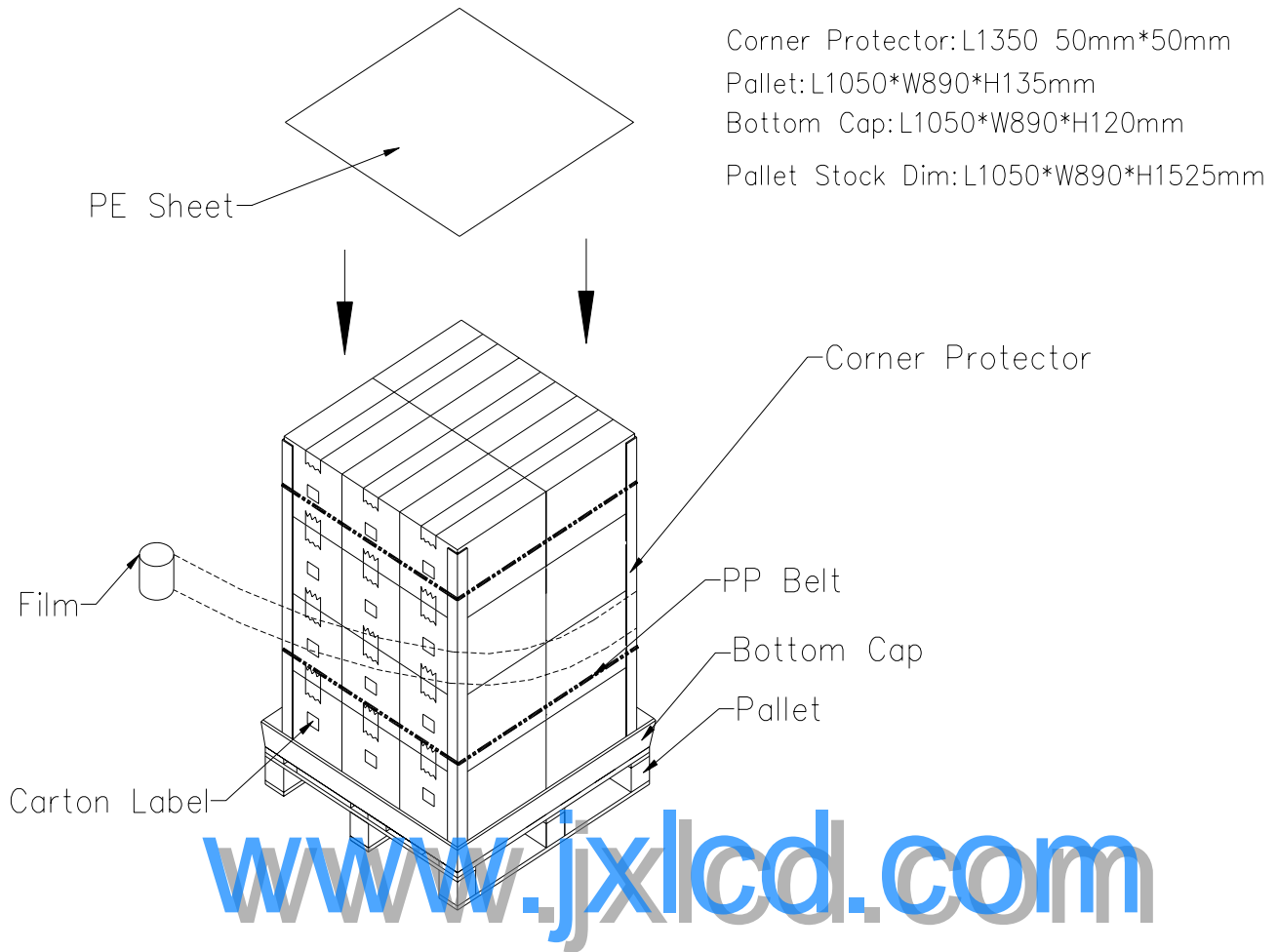
Figure. 10-2 Packing method
