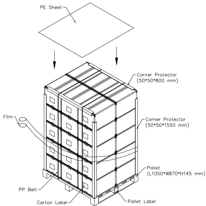
Figure. 9-2 Packing method
