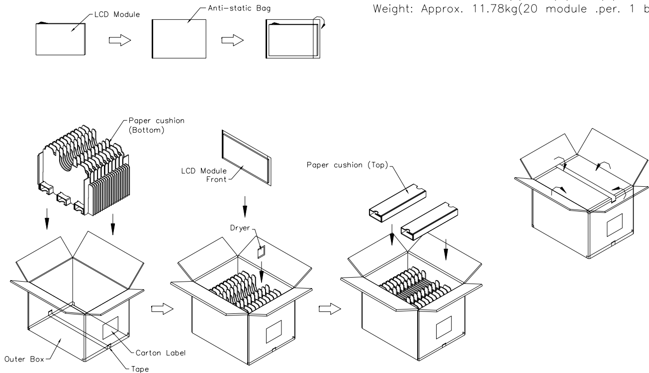
Figure. 9-1 Packing method
