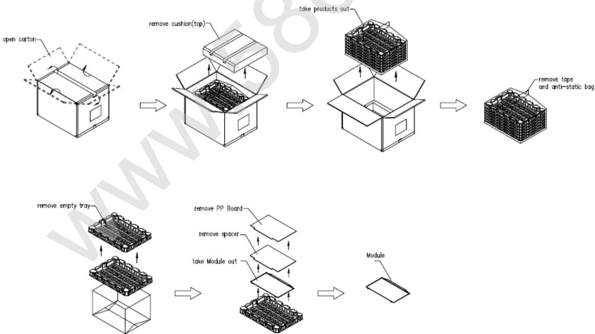
Figure. 7-3 Un-Packing method
