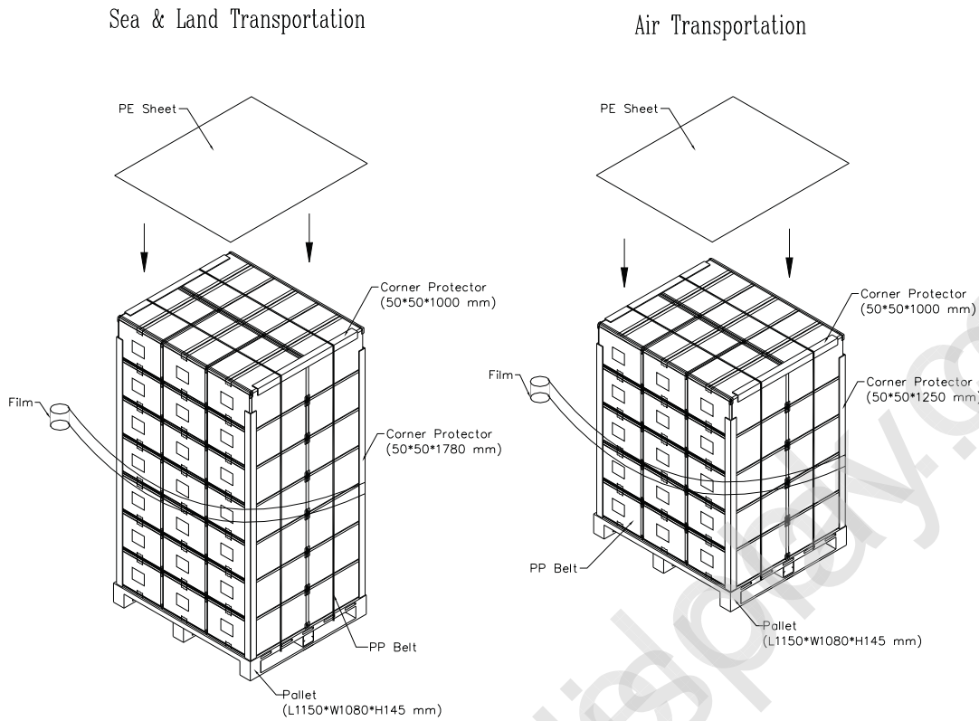
Figure. 7-3 Packing method
