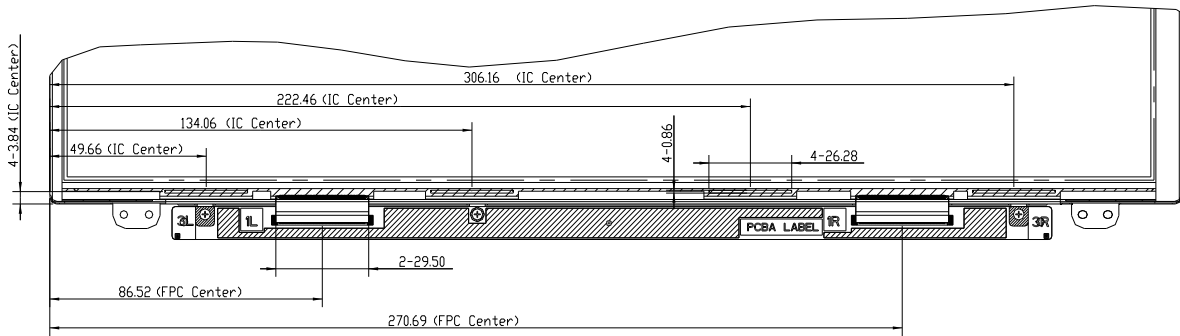
SECTION A-A SCALE 5:1
