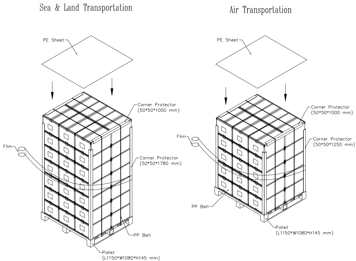
Figure. 7-2 Packing method
