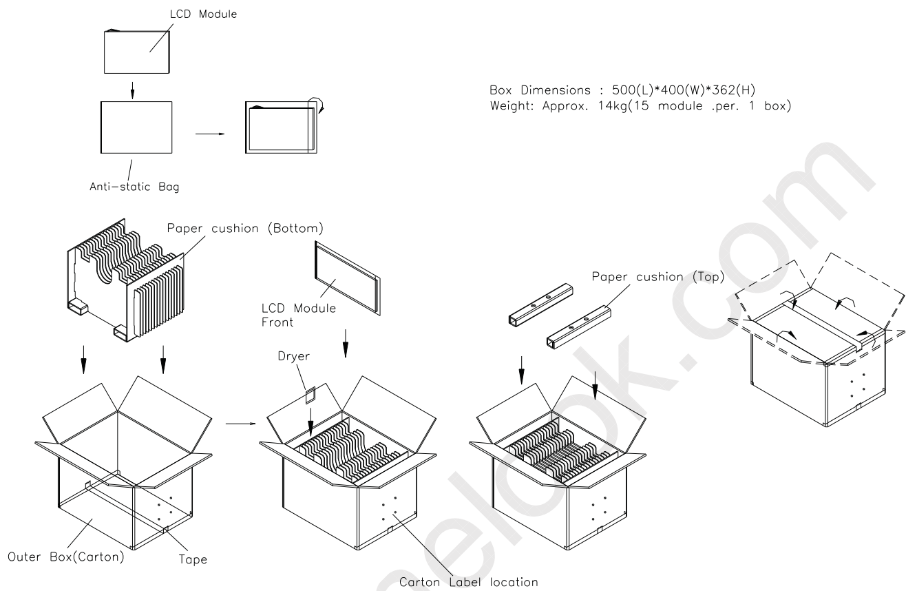
Figure. 9-1 Packing method
