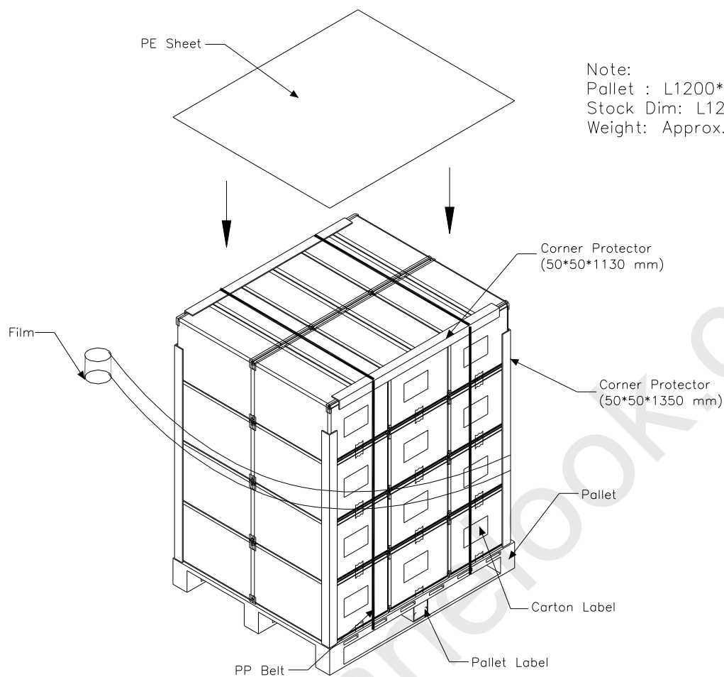
Figure. 9-3 Packing method
