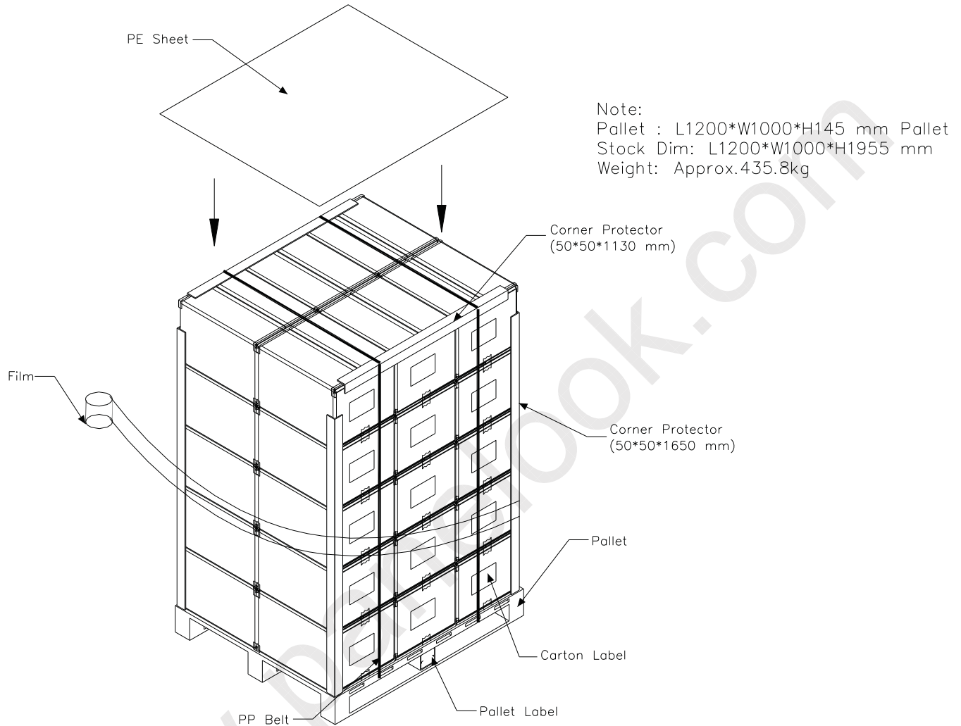
Figure. 9-2 Packing method
